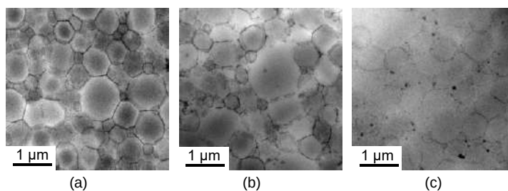
Figure 1. TEM images of (a) DPNR-graft-PSS(1.0), (b) DPNR-graft-PSS(0.75), (c) DPNR-graft-PSS(0.50).
