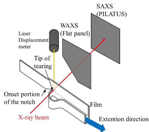
Fig.1 Schematic illustration of SAXS/WAXS simultaneous measurements along with tearing of the notched film.
