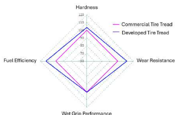
Figure 2. Normalized graph comparing key properties of the developed tread compound with the commercial tire tread used by the Military
