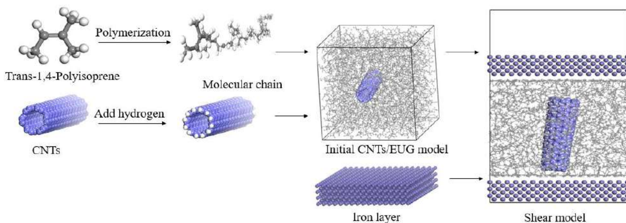
Figure 1. Construction process of molecular models of CNTs/EUG composites
