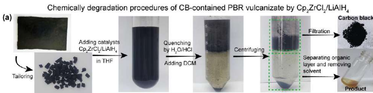
Figure 1. General procedures for chemical degradation of CB-contained polydiene vulcanizate by \text{Cp}_2\text{ZrCl}_2/\text{LAH} (reaction conditions: 0.535g PBR vulcanizate (0.0092 mol C=C bond), [\text{Cp}_2\text{ZrCl}_2]/[\text{LAH}]/[\text{C}=\text{C}] = 0.025/0.0/1 , 60 °C, 20ml THF, 20 min).
