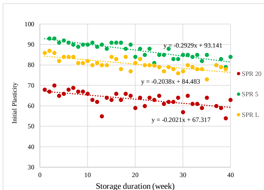
Figure 2. Initial Plasticity vs. Storage Duration for Standard Philippine Rubber Grades
