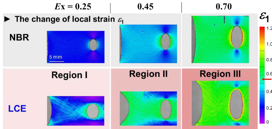
Figure 4 Distribution of major principal strain \varepsilon_1 .
