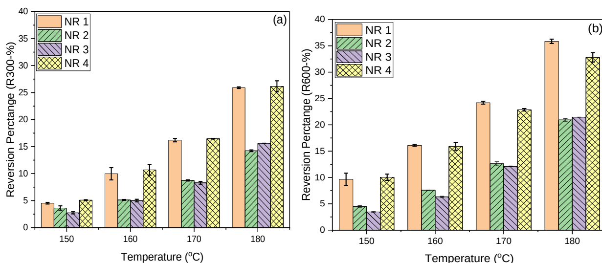
Figure 1. The reversion percentage of NR series blends at R 300 (a) and R 600 (b) times are at 150 °C, 160 °C, 170 °C, and 180 °C.
