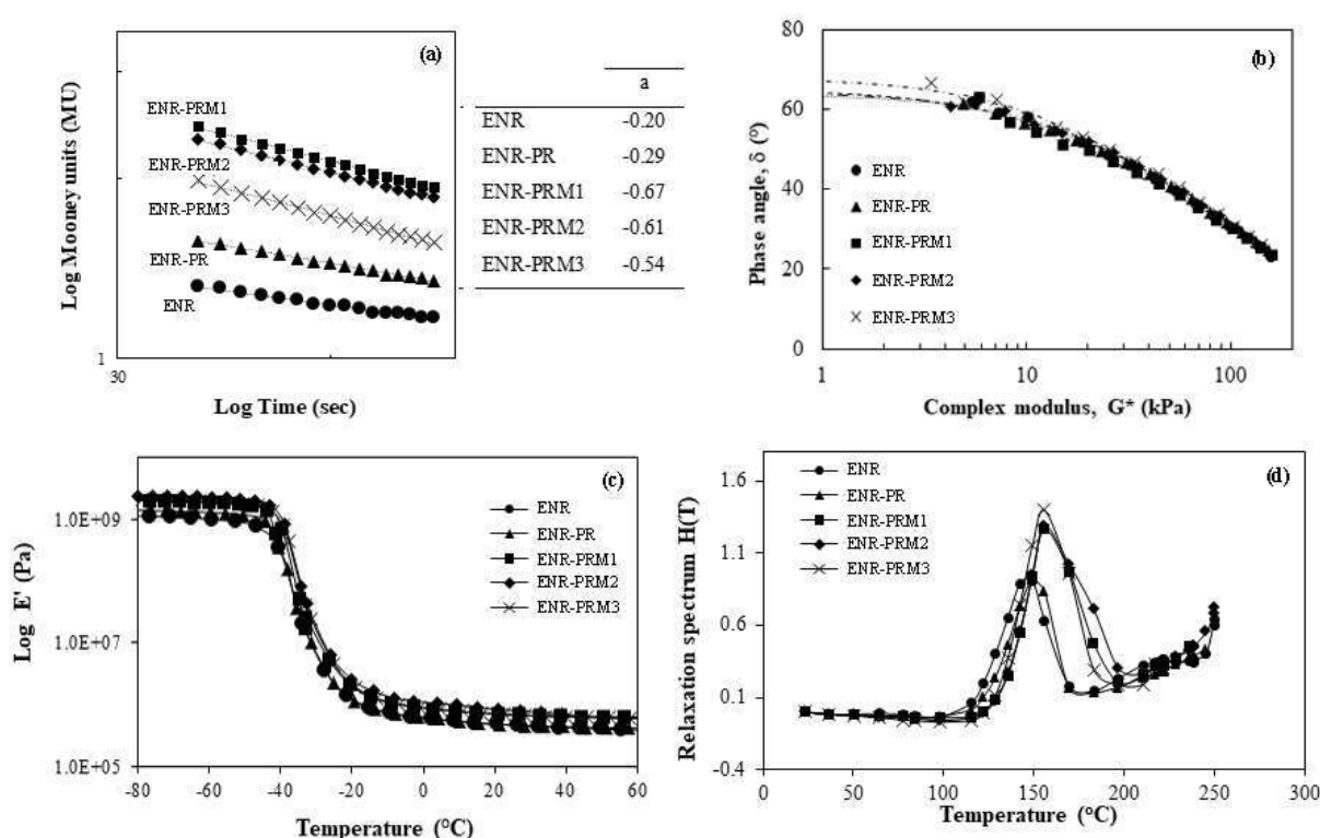
Figure 1. Dynamic behavior and relaxation properties of the uncured and cured ENRs
