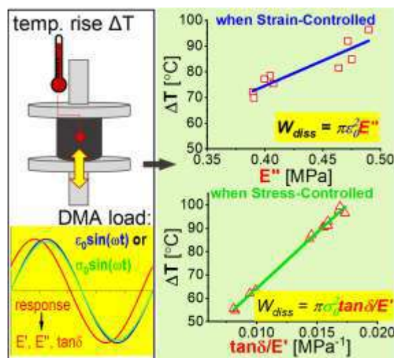
Figure 1. The rubber heat build-up amplitude \Delta T due to hysteresis exhibits a distinctive dependency on viscoelasticity: (upper plot) at strain-controlled deformation, \Delta T is determined by E'' ; (lower plot) while at stress-controlled mode, \Delta T correlates to \tan\delta/E' . [3]
