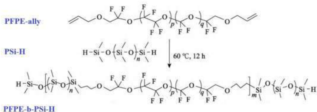
Figure 1. Synthesis process and structure of silicone-modified PFPE polymer chain (PFPE-b-PSi-H)
