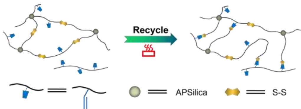
Figure 1. x-APSilica/IPU polyurethane rubber composite system recyclable enhancement mechanism
