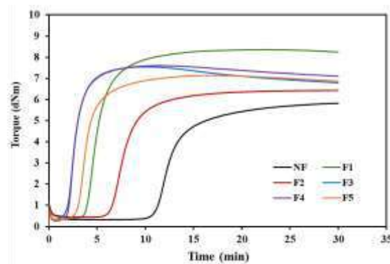
Figure 1. Cure characteristics of different types of fly ashes filled NR at 150°C
