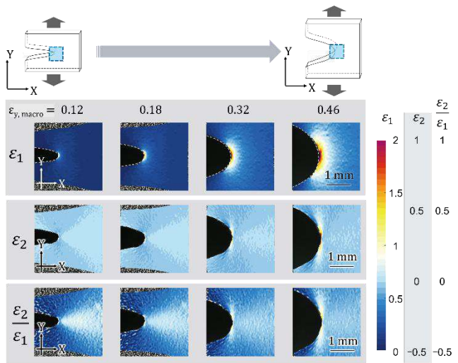
Fig. 4. Development of strain fields around a crack-tip during crack opening.
