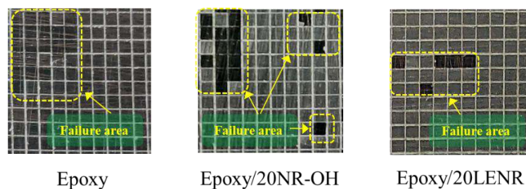
Figure 1. Examples of cross-hatch adhesion test of waterborne epoxy resin without and with functionalized natural rubber; Epoxy/20NR-OH and Epoxy/20LENR for 1 day of curing time at room temperature
