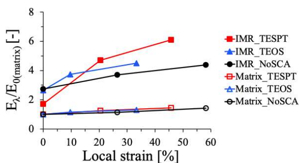
Figure 2. Ratios of elastic modulus of matrix and intermediate-modulus region (IMR) at each local strain to elastic modulus of matrix in the unstretched state.
