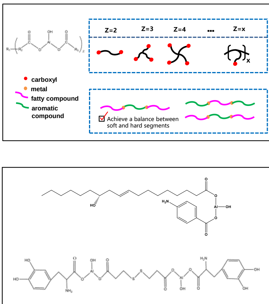
Figure 1. Structural Design of Aluminum Soap
