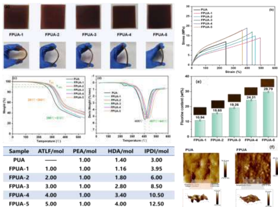
Figure 2. (a) Effect of ATLTF content on hardness of FPUA. (b) Effect of ATLTF content on the mechanical properties of FPUA. (c) TGA thermograms of PUA and FPUAs. (d) DTG thermograms of PUA and FPUAs. (e) Effect of ATLTF content on the fluorine content of FPUA. (f) AFM images of PUA and FPUA.
