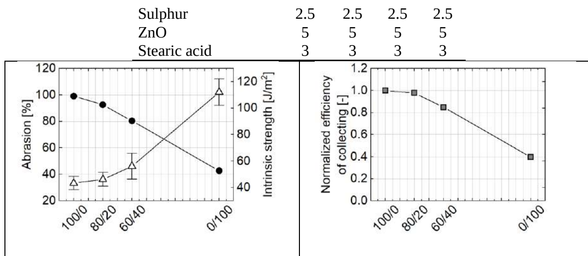
Figure 1. The graphs on the left illustrate the abrasion resistance (circles) and the intrinsic strength (triangles) of rubber compounds with various NR/BR ratio, while the graph on the right shows the efficiency of collecting abraded particles (squares)
