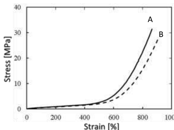
Figure 6 Stress-strain curves for latex-mixed natural rubber vulcanizate (A) and mechanically mixed natural rubber vulcanizate (B).
