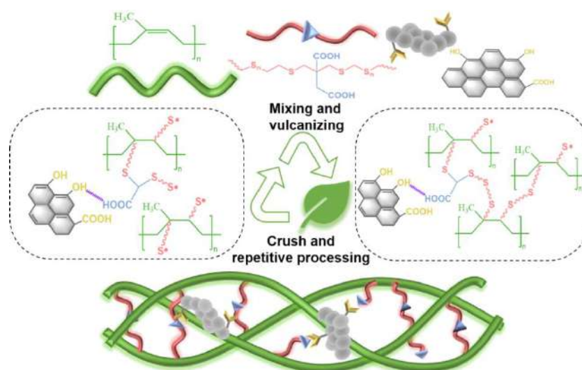
Figure 2. Mechanism of recycling processing
