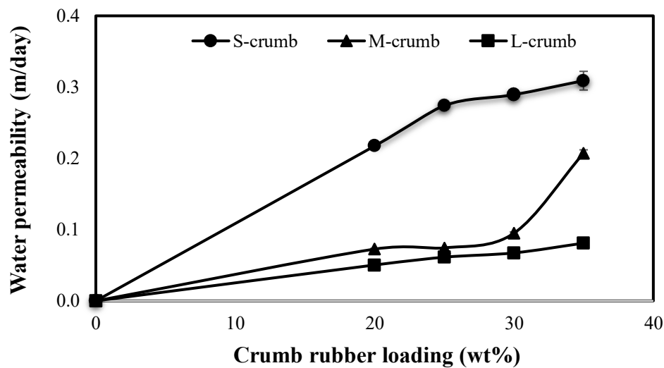
Figure 2. Water permeability of soil amended with different crumb sizes and loadings
