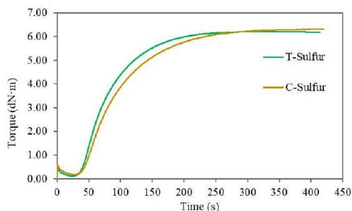
Figure 2. Cure curves of NR compound with various sulfur.
