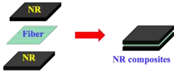
Figure 2. Preparation of sandwich-structured rubber composites
