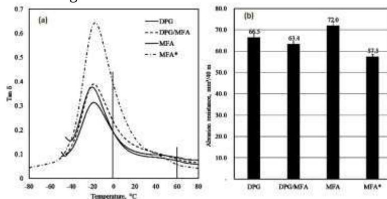
Figure 2. Tan \delta vs temperature (a) DIN volume loss (b) of silica-filled tire tread vulcanizate
