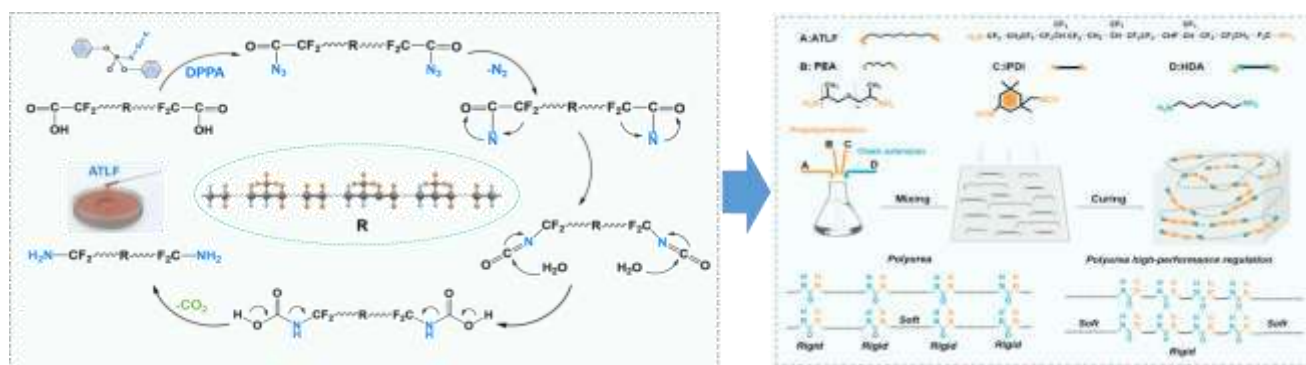
Figure 1. Synthesis mechanisms of ATLFF and high-performance FPUA
