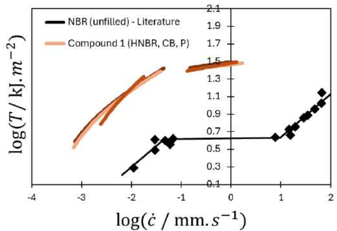
Figure 3: Tearing energy versus crack speed. Results for unfilled NBR [4] and Compound 1 tested using the continuously increasing strain method are shown, including repeat measurements.
