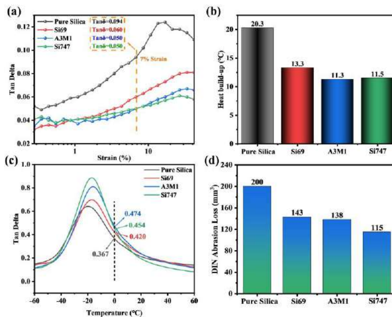
Figure 2. (a) Tan Delta-strain curves at 60°C, (b) Heat build-up, (c) DMA curves and (d) DIN abrasion loss of silica/NR composites.
