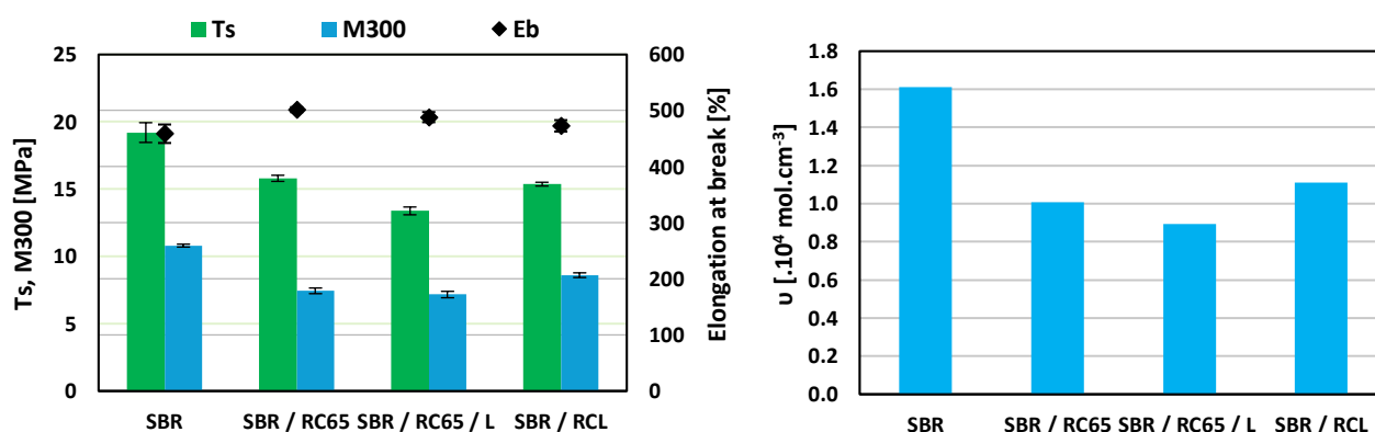
Figure 1. Mechanical properties (a) tensile strength T_s , modulus M_{300} and elongation at break E_b and (b) cross-link density \nu of composites
