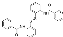
Figure 1. Chemical Structure of the used DA: 2,2'-Dibenzamido diphenyl disulfide
