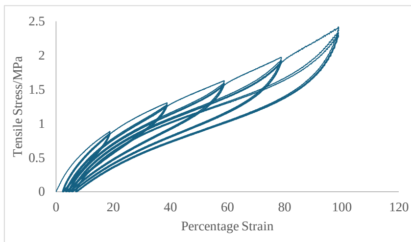
Figure 2. Quasi-static cyclic stress-strain testing of a model carbon black-filled car tyre rubber compound under tension
