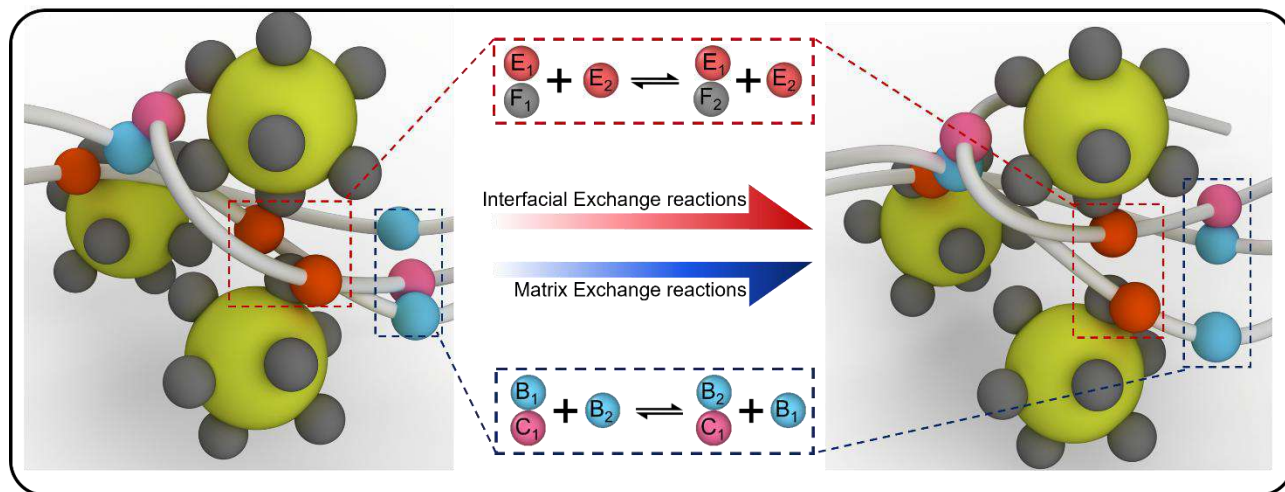
Figure 1. Bond swap mechanism of PVNs. There are two types of dynamic bond swaps: interfacial bond swaps (occur between the reactive beads on the vitrimer and on the NPs, highlighted by the red dashed box) and matrix bond swaps (occur between the active beads of vitrimer itself, highlighted by the blue dashed box). Other unreactive beads on the polymer chain are indicated by white lines.
