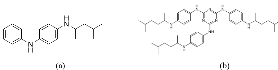
Figure 1. Chemical structures of (a) 6PPD and (b) Durazone D37.
