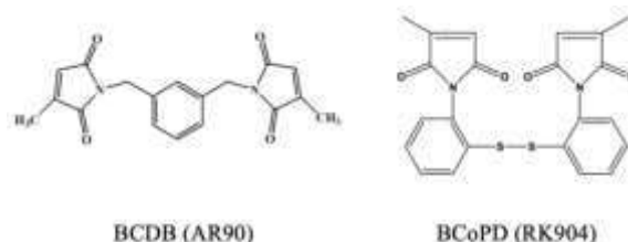
Figure 1. Chemical structures of anti-reversion agents AR90 and RK904
