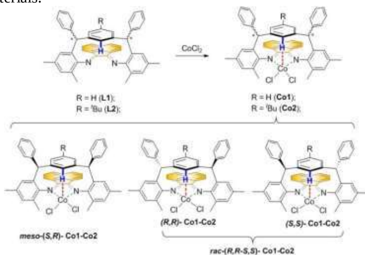
Figure 1. Synthetic procedure for the \alpha -diimine cobalt complexes Co1-Co2 bearing axial anagostic interaction \text{Co}\cdots\text{H}-\text{C} .
