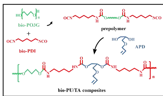
Figure 1. Fabrication routes of bio-PU/TA composites
