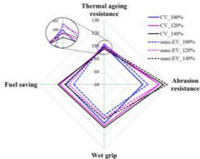
Figure 1. Normalized graph of tire performance and thermal ageing resistance at various relative curative contents and sulfur vulcanization systems
