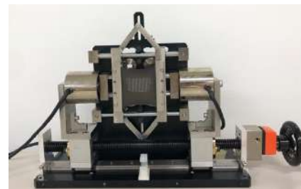
Fig 1. High-speed shrinkage device.
