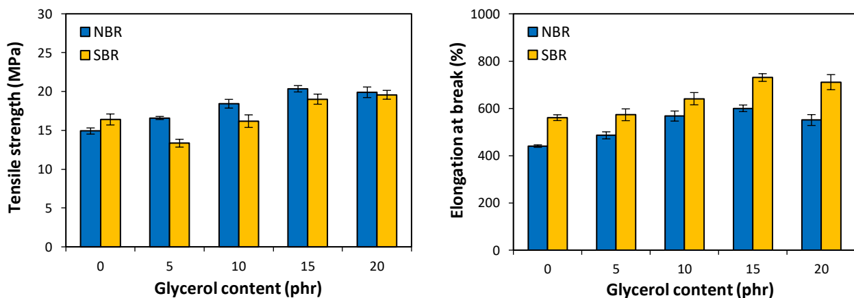
Figure 2. Influence of glycerol content on tensile strength (left) and elongation at break (right) of composites
