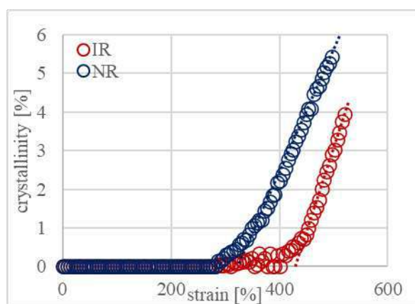
Figure 1. Crystallinity as a function of strain
