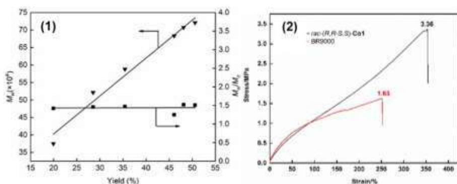
Figure 2. (1) The dependence of molecular weights and polydispersities on the monomer conversions; (2) stress-strain curves of UHMWPBd and BR9000.
