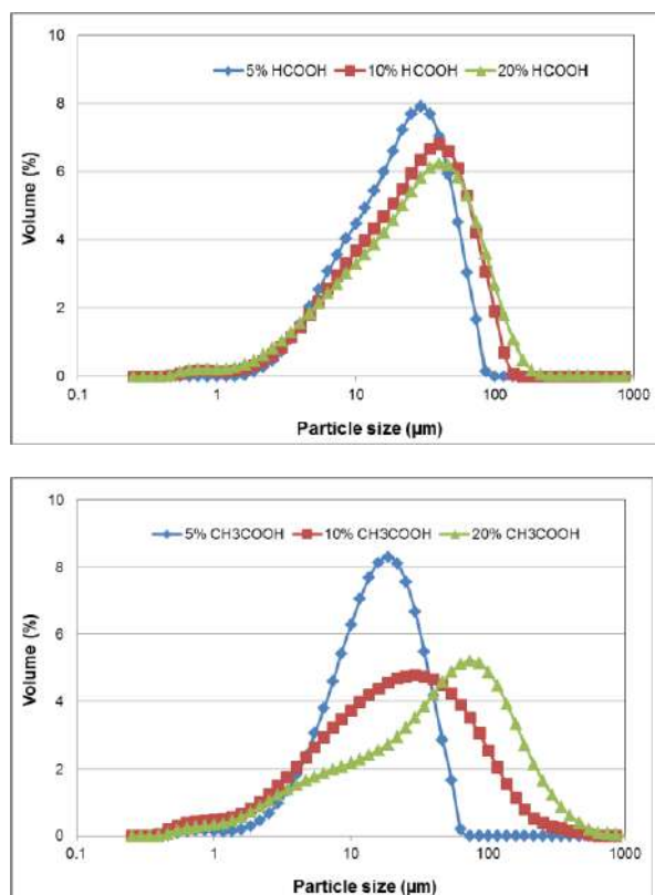
Figure 1: Particle size distribution of precipitated silica obtained from treating sodium silicate solution with various types and concentrations of acid.
