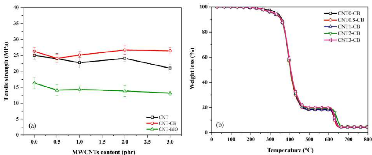
Figure 2. (a) Tensile strength and (b) TGA thermogram of rubber composites
