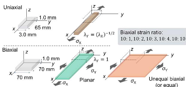
Fig. 1 Schematics of several types of deformation: uniaxial, planar, unequal biaxial (nominal strain ratio \epsilon_y/\epsilon_x = 0.1, 0.2, 0.3, 0.4 ), equi-biaxial.
