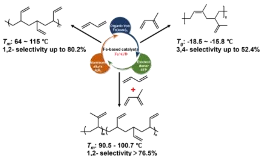
Figure 1. Homo-polymerization and copolymerization of butadiene and isoprene
