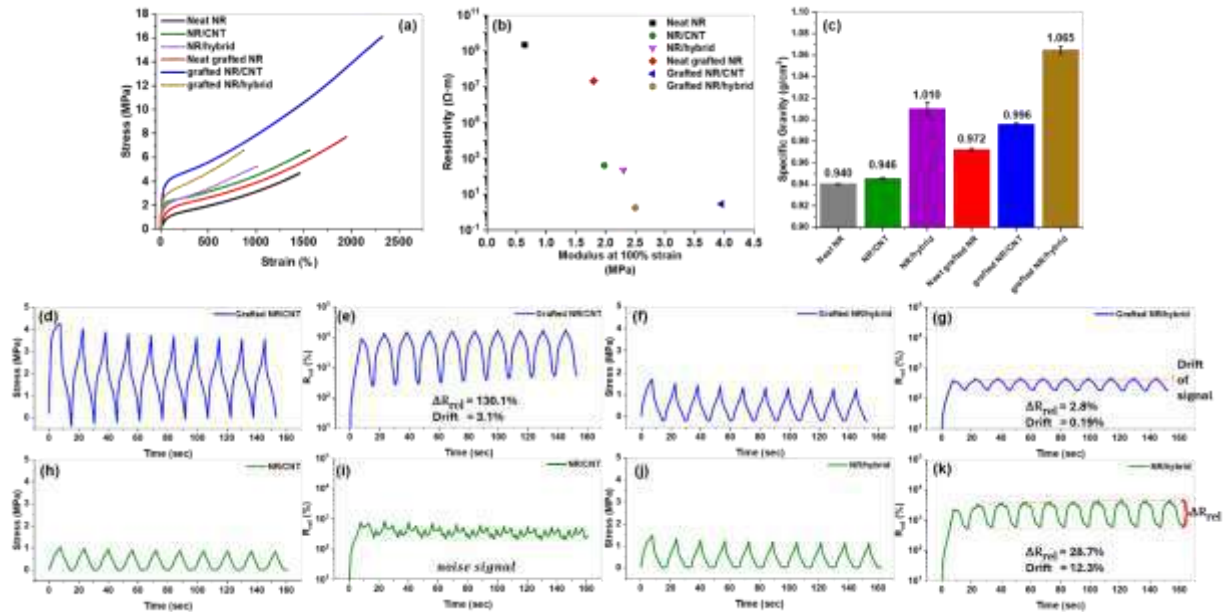
Figure 1. The stress-strain curves (a), resistivity (b), specific gravity (c) and relation of stress and time (d-k) of the composites with the R_{rel} as a function of time during the dynamic tests in 10 cycles at 0-100 % strain.
