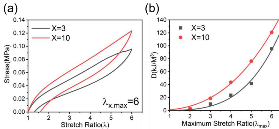
Figure 1. (a) Tensile loading-unloading cycles of PAAm-fCNT-2 ( X=3 and 10) at \lambda_{x,max}=6 and (b) the corresponding dissipated energies at different \lambda_{x,max} .
