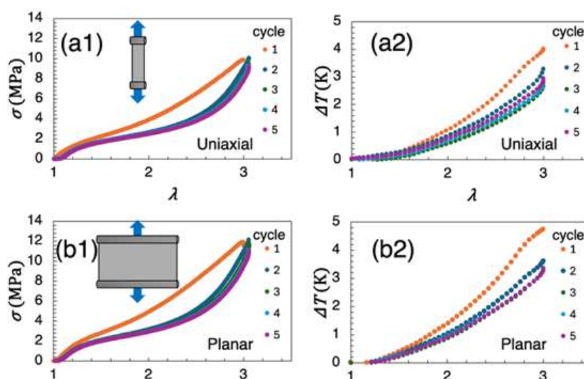
Fig.1 (a1, b1) Engineering stress and (a2, b2) surface temperature increase against elongation for CB-filled SBR in loading processes of multiple loading-unloading cycles by uniaxial stretch(a1, a2) and planar stretch(b1, b2)
