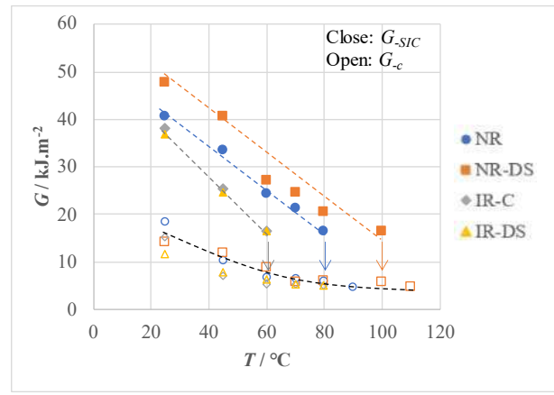
Figure 2. G_{SIC} and G_c as a function of T at 0.5s -1
