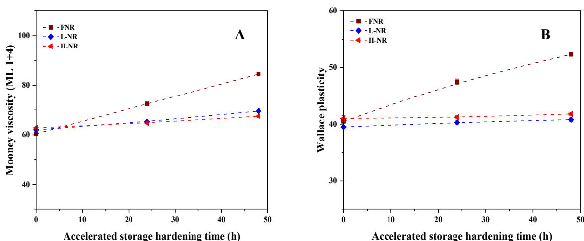
Figure 1. Changes in Mooney viscosity (A) and Wallace plasticity (B) of FNR, L-NR, and H-NR during accelerated storage hardening.
