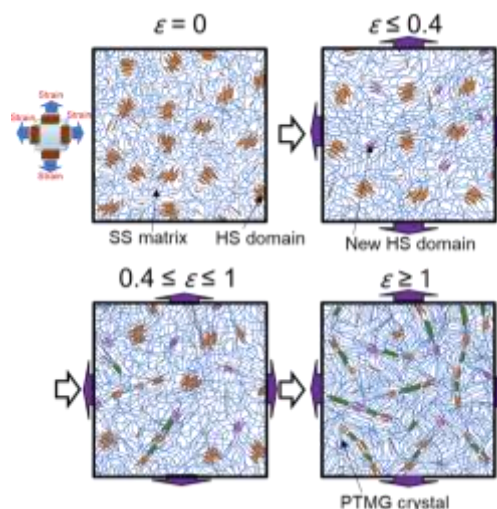
Figure 4. Schematic illustration of the molecular chain structure of SPU during equi-biaxial deformation.
