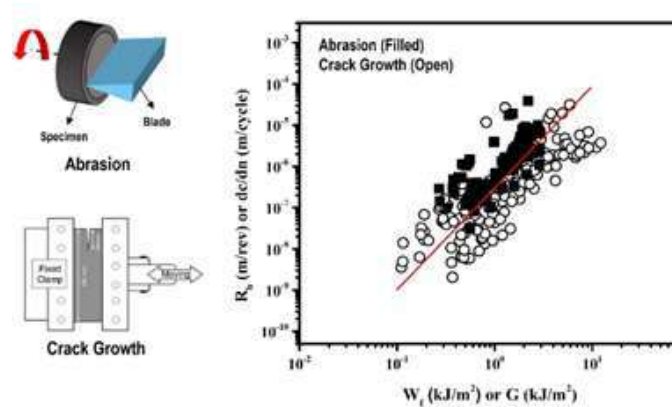
Figure 2. Correlation between abrasion and crack growth behavior [5].
