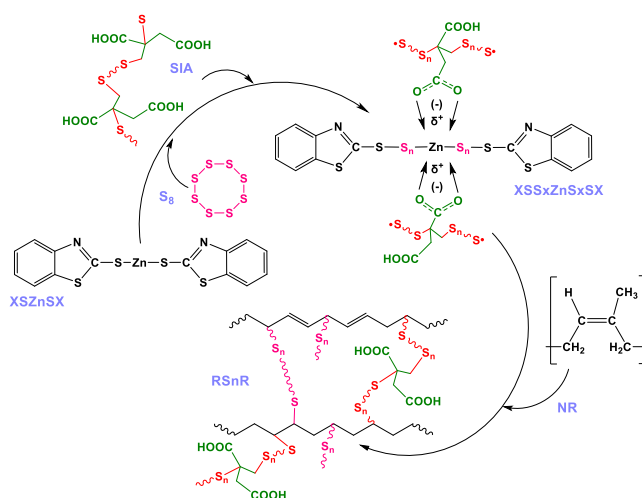
Figure 1. The mechanism of co-vulcanization
