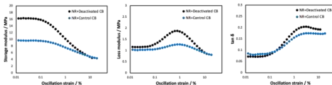
Figure 2. The storage modulus( E' ), loss modulus( E'' ) and \tan \delta at 60°C of rubber with different surface activity of carbon black, respectively.
