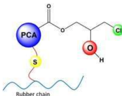
Figure 1. Illustration of the proposed epichlorohydrin-modified reclaimed rubber product (FD-GTRECH).
