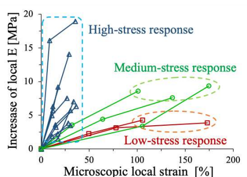
Figure 3. The local strain-local stress relationship in the specific regions for silica/SBR with TESPT.
