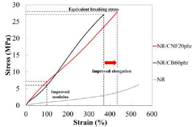
Figure 3. Tensile test
