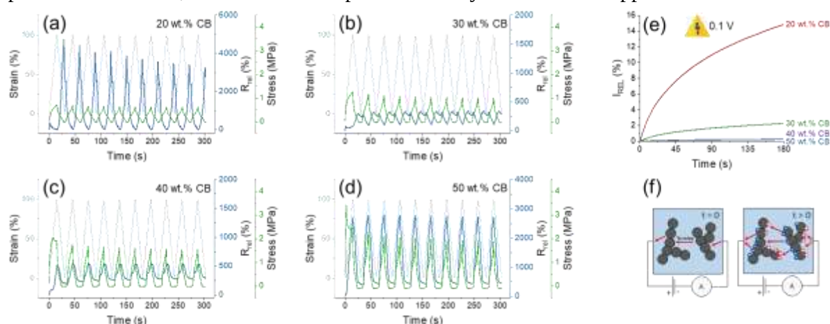
Figure 1. Dynamic mechano-electrical behavior of a TPS Shore 22A elastomer mixed with (a) 20 wt.% CB, (b) 30 wt.% CB, (c) 40 wt.% CB, and (d) 50 wt.% CB. (e) Polarization experiments under a constant applied voltage of 0.1 V. (f) Schematic illustration of the proposed polarization mechanism.
