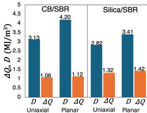
Fig.2 Heat generation difference between the first and fifth loading ( \Delta Q ) and mechanical energy dissipation ( D ) for each specimen during uniaxial and planar stretch cycles.
