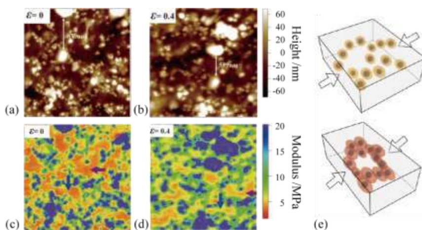
Figure 2. In-situ AFM height images of CB-filled IR at macroscopic compressive strains \varepsilon = (a) 0 and (b) 0.4. (c) (d) The corresponding modulus images. The scan size is 3.0\ \mu\text{m} . (e) Schematic diagram of the formation of stress network.
