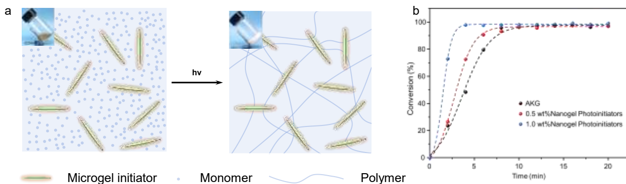
Figure 1. (a) Nanogel photoinitiator initiates polymerization under visible light, (b) Photopolymerization kinetics of acrylate monomers.
