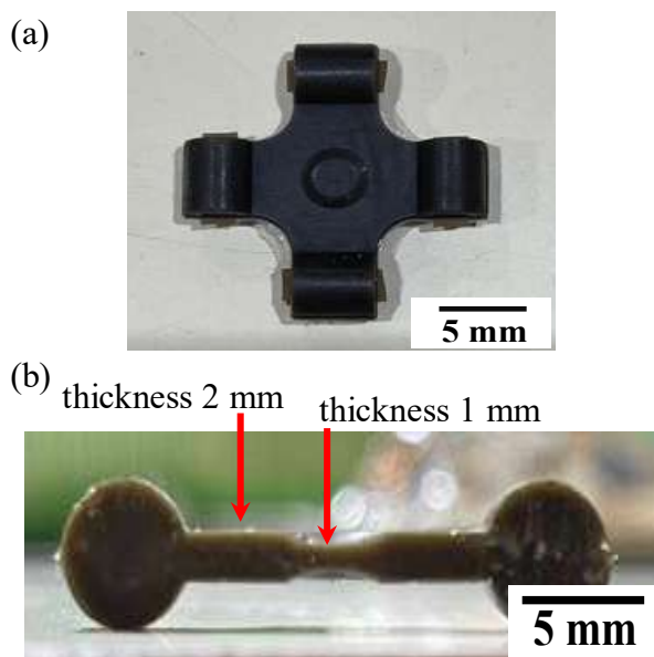
Fig.1. Cross-shaped natural rubber specimen for biaxial elongation.
