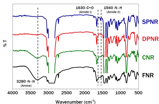
Figure 1. FTIR spectra of FNR, CNR, DPNR, and SPNR.
