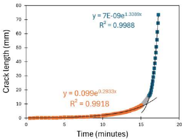
Figure 2: Crack length versus time for a sample subjected to continuously increasing strain. Curves are fitted to the slow crack growth and transition crack speed regions.
