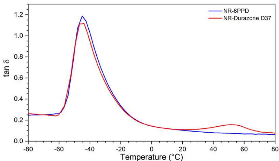
Figure 2. DMTA results of CB-filled NR vulcanizates containing 6PPD and Durazone D37.
