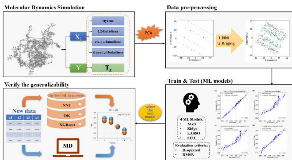
Figure 1. Schematic illustration of the integrated MD-ML workflow for predicting the glass transition temperature of SSBR.
