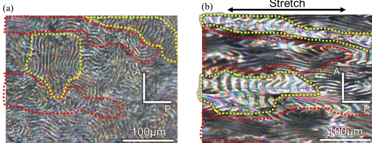
Fig.3 FP textures and of FP-CE in the (a) undeformed and (b) stretched ( \epsilon_x=0.9 ) states. The yellow dotted area depicts a domain with the initial stripes almost perpendicular to the stretching axis.
