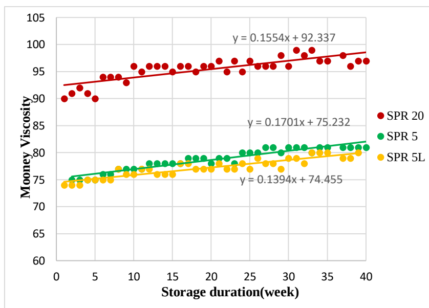
Figure 1. Mooney Viscosity vs. Storage Duration for Standard Philippine Rubber Grades
