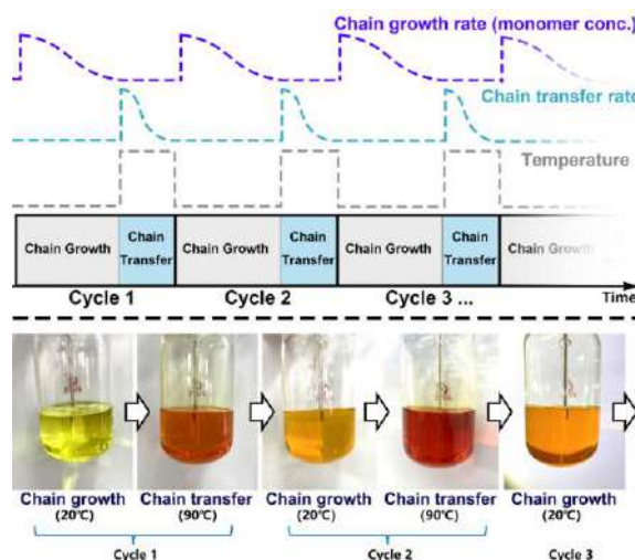
Figure 1. Schematic illustration of the pulsed chain transfer polymerization process
