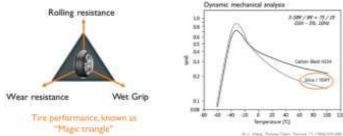
Fig. 2: Magic triangle and rolling resistance indicator of silica- and carbon black based tire treads.
