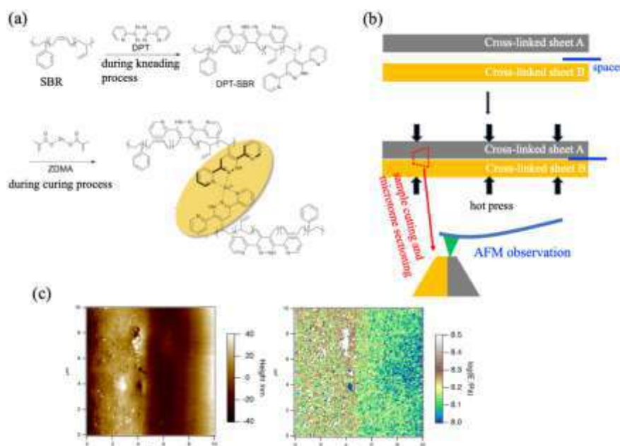
Figure 1. (a) Schematic illustration of the reaction process used to prepare DPT-SBR/ZDMA composites. 2 (b) Schematic of the adhesive sample preparation for AFM experiments. (c) Height and elastic modulus (in log scale) maps measured using QNM method across the interface between two rubber sheets.
