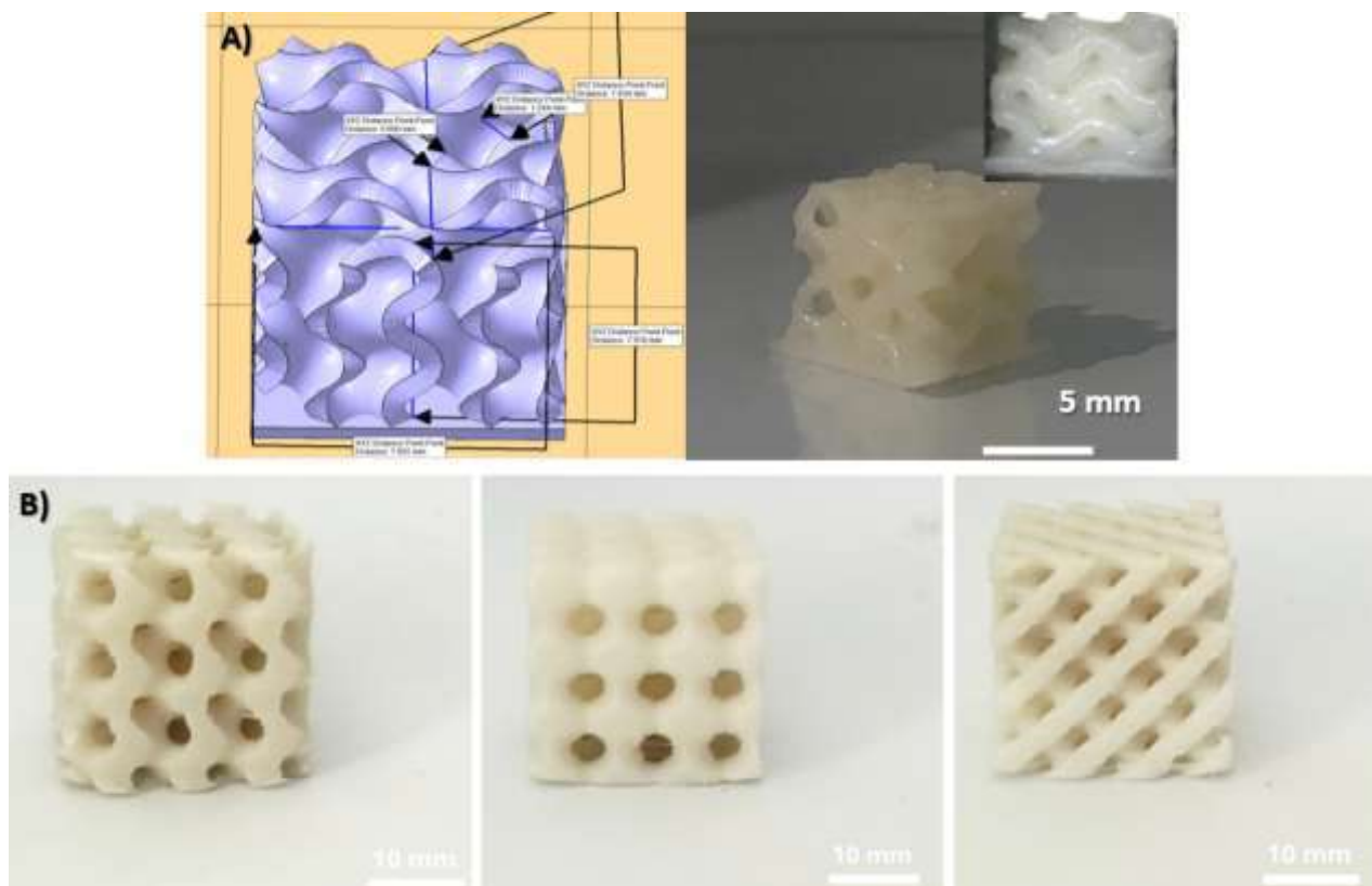
Figure 1. (A) Computer-aided design (CAD) model of a gyroid structure (left), and the corresponding 3D-printed construct using the photocurable natural rubber latex (PNLR) formulation (right) and (B) Photographs of 3D-printed lattice structures based on TPMS geometries, fabricated using PBS/ENR composite filaments via FDM. From left to right: Gyroid, Primitive, and Diamond structures.
