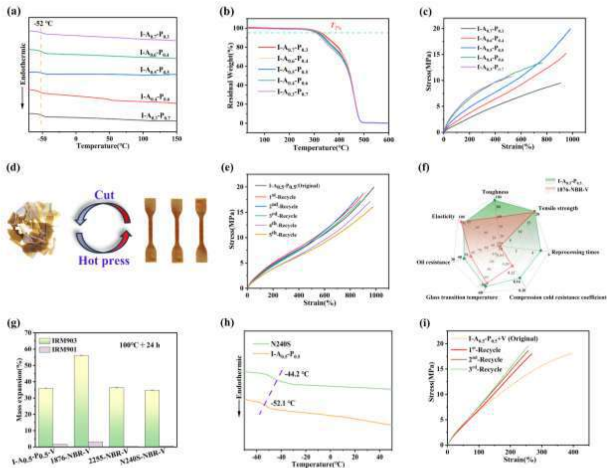
Figure 1. (a) DSC curves, (b) TGA curves, (c) Stress–strain curves of IPDI-ATBN-PPD. (d) Photograph of I-A 0.5 -P 0.5 recycled dumbbell strip. (e) Stress–strain curves of original and recycled samples. (f) Comparison of I-A 0.5 -P 0.5 and 1876-NBR-V. (g) Oil resistance of I-A 0.5 -P 0.5 -V, 1876-NBR-V, 2255-NBR-V, and N240S-NBR-V. (h) DSC curves of N240S and I-A 0.5 -P 0.5 . (i) Stress–strain curves of original and recycled samples.
