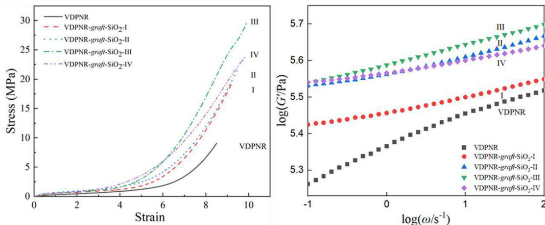
Figure 2. Stress-strain curves and storage modulus versus the frequency for vulcanized DPNR-graft-SiO 2
