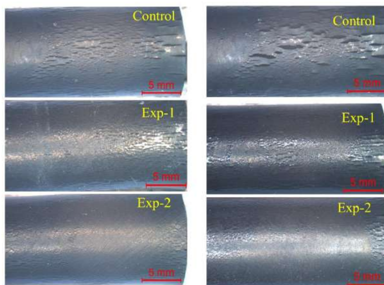
Figure 1. Optical Microscopy images of control with wax, Exp-1 for partial substitution and Exp-2 representing complete substitution of wax after 24hr (LHS) and 72hr (RHS) ozone exposure.
