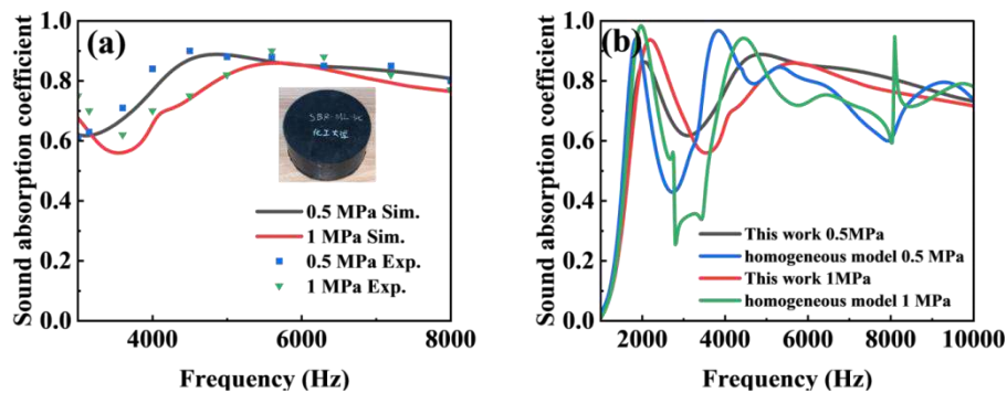
Figure 3. (a) Simulated vs. experimental sound absorption coefficients; (b) This work vs. homogeneous material model
