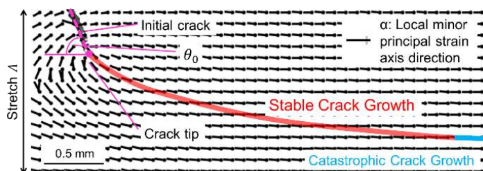
Figure 2. 2D distribution of local minor principal strain axis direction at crack-growth onset for \theta_0 = 72.8^\circ . The data are shown in the coordinate system before deformation. The red line represents the path of stable crack growth.
