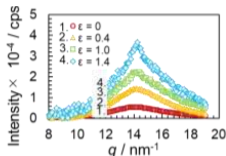
Figure 3. WAXD profiles of SPU during equi-biaxial deformation.
