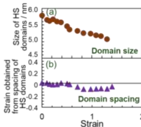
Figure 2. (a) HS domain size and (b) HS domain spacing of SPU during equi-biaxial deformation.
