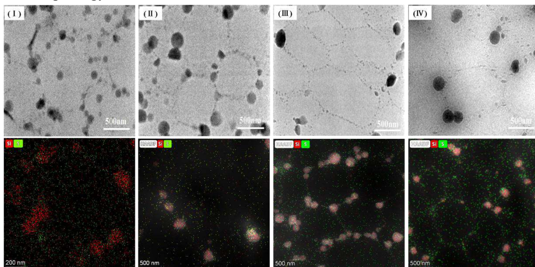
Figure 1. TEM and EDS images for vulcanized DPNR-graft-SiO 2
