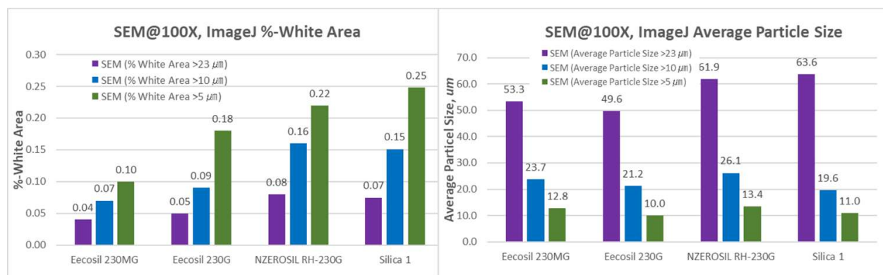
Figure 7. %-White areas (left) and Average particle sizes (right) of four difference silica treads.
