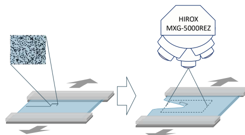
Fig. 2 Schematics of quantification of two-dimensional strain distributions during elongation of a specimen with a hole.
