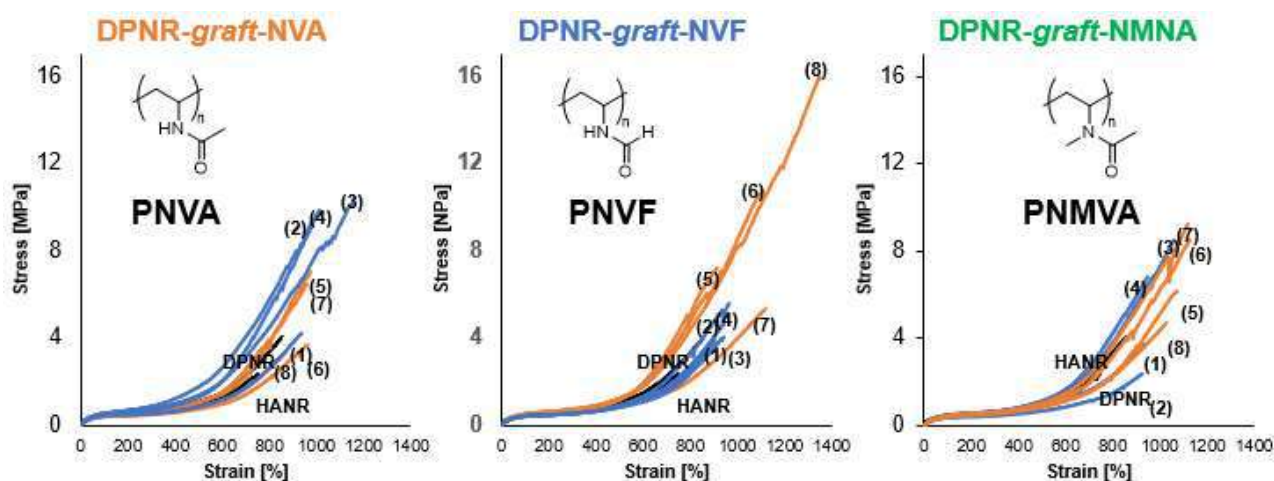
Figure 2. Tensile tests of DPNR-graft-poly( N -vinylamide)s.
