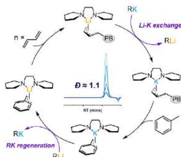
Figure 1. Mechanism of pulsed chain transfer polymerization
