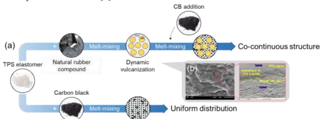
Figure 2. (a) Schematic of the fabrication process for uniformly dispersed TPS/CB and co-continuous TPS/NR/CB compounds. (b) SEM image showing the morphology of the TPS/NR/CB compound.
