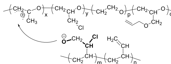
Figure 3. Crosslinking reaction
