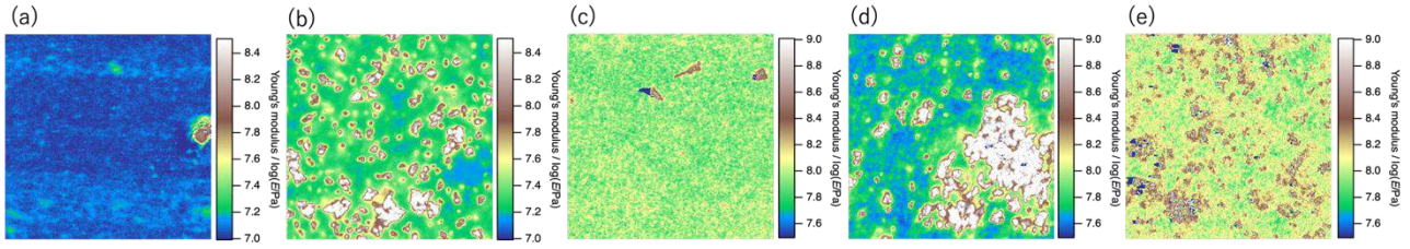
Figure 1. Young's modulus image obtained by AFM. (a) SBR, (b) SBR+Silica, (c) SBR+MPR, (d) SBR+MPR+silica and (e) SBR+MPR+Silica with doubled kneading time. Scan size is 2.0 \mu\text{m} .
