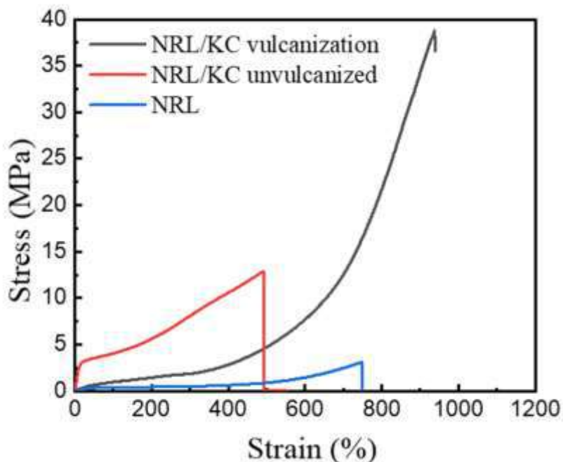
Figure 1. Mechanical performance of NRL and NRL/k-carrageenan composites (NRL/KC).
