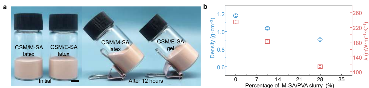
Figure 1. Compounding performance of CSM latex with E-SA/PVA and M-SA/PVA slurries, scale bar is 1cm
