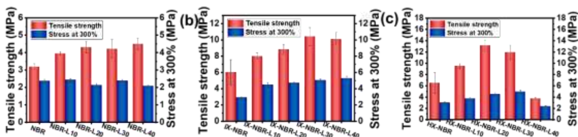
Figure 3. Maximum stress and 300% modulus at a fixed extension of (a) NBR-L, (b) IX-NBR-L, and (c) HX-NBR-L.
