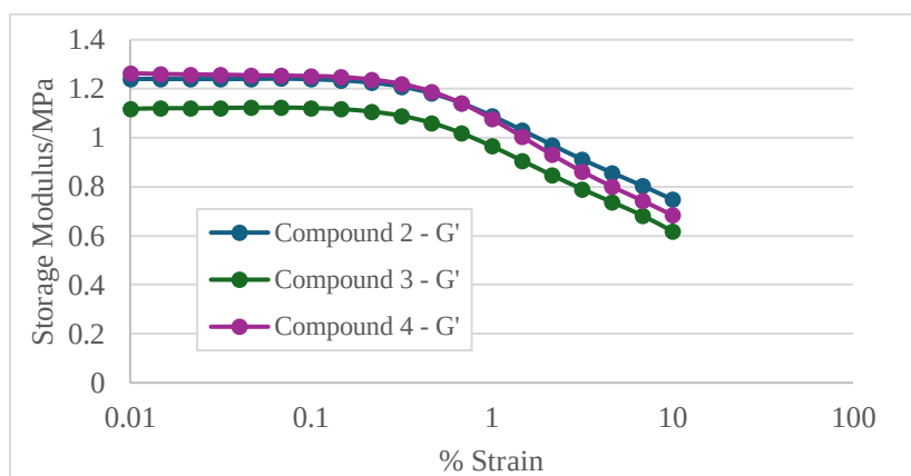
Figure 3. Effect of coupling agents on Payne effect as measured by Shear Sandwich DMA
