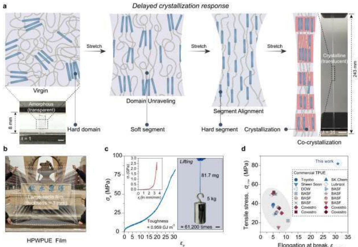
Figure 1. Microstructural changes in our HPWPUE during the DCR process and their mechanical properties
