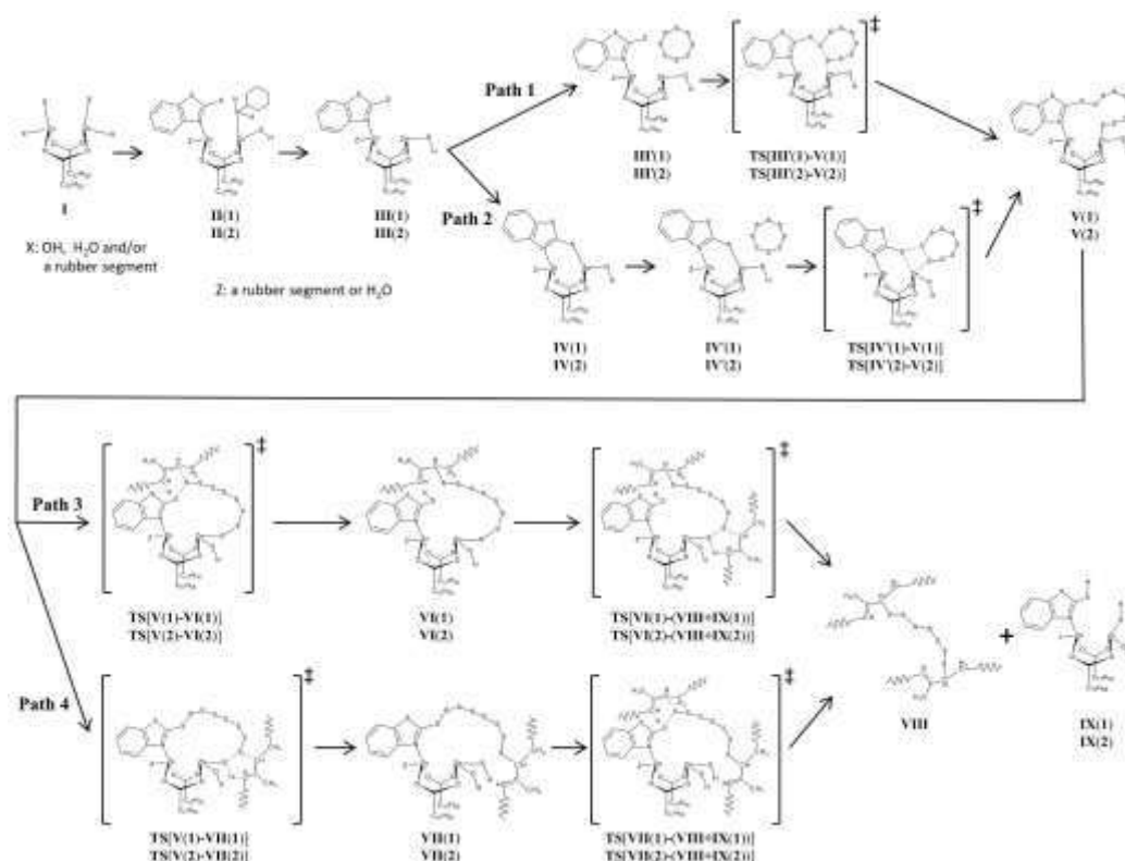
Figure 1. The highly possible reaction scheme of the N -cyclohexyl-2-benzothiazole sulfenamide-accelerated vulcanization to generate sulfur cross-linked isoprene rubber.
