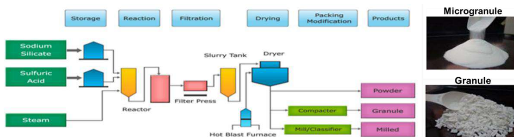
Figure 4. Manufacturing Process of Amorphous Silica by Sodium Silicate reaction with Acid.
