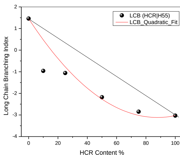
Figure 2. Variation of LCB index value of CO/HCR blends with HCR content
