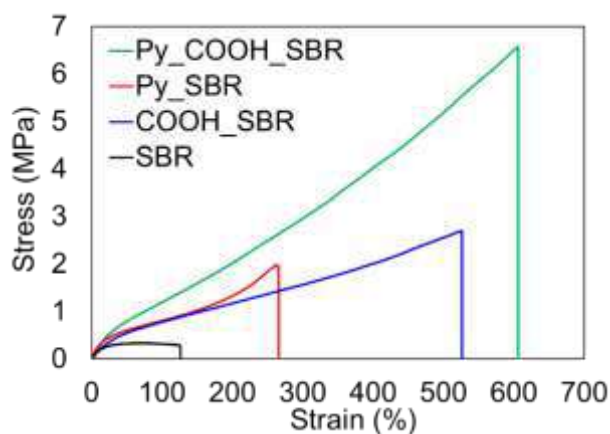
Figure 1. Stress-strain relation of pyridine and COOH modified SSBR and its mixture.
