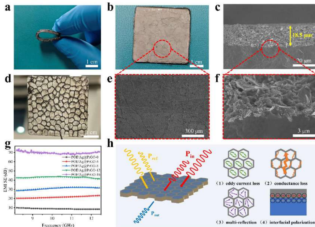
Figure 2. (a) The digital image exhibiting the bending performance of POE/Ag@PrGO composites; (b and e) The digital and SEM images of POE/Ag@PrGO composites; (c and f) SEM images of the cross-section of POE/Ag@PrGO composites; (d) The digital image of POE/Ag@PrGO composites after the conductive layers on the surface have been polished; (g) The EMI SE of POE/Ag@PrGO composites in the X band; (h) The EMI shielding mechanism of POE/Ag@PrGO composites.
