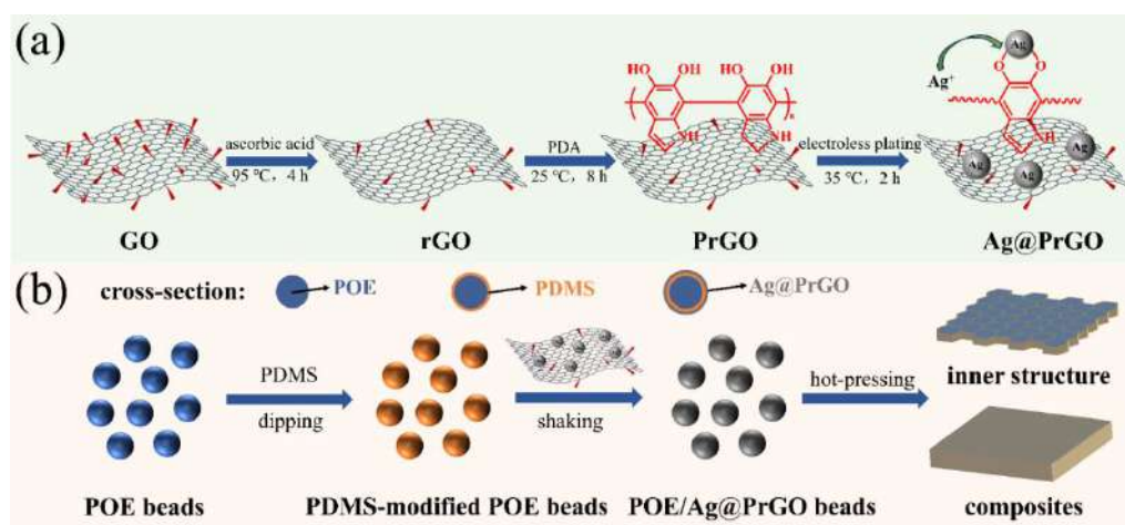
Figure 1. Fabrication process for the (a) Ag@PrGO fillers and (b) POE/Ag@PrGO composites.
