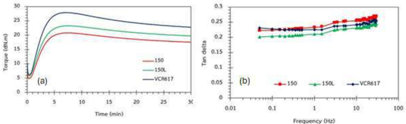
Figure 3. Cure curves and tan delta at 60 °C of filled-NR/BR blends with different BR grades
