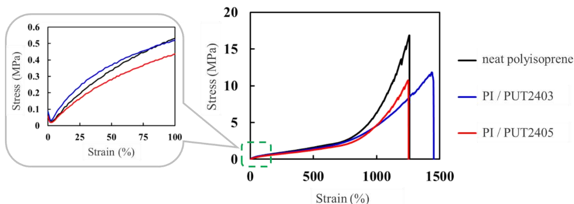
Figure 1. Stress-strain curves of polyisoprene blended with urethane compounds.
