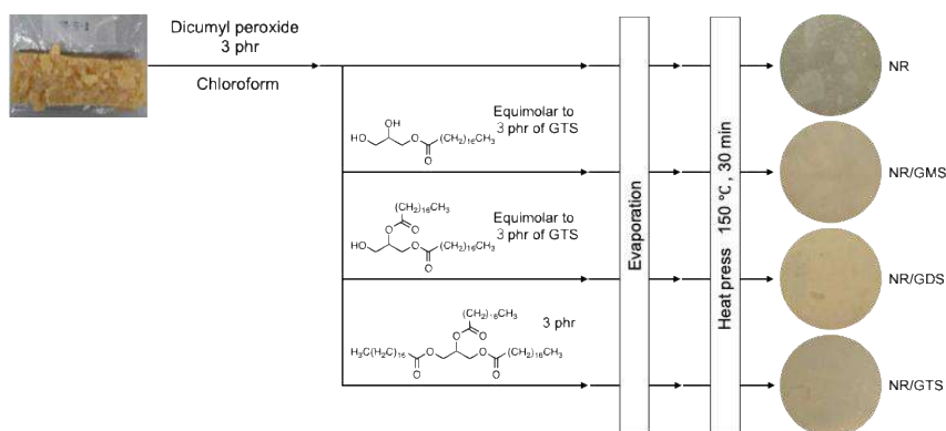
Figure 1. The sample preparation process of NR, NR/GMS, NR/GDS, and NR/GTS.
