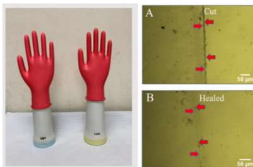
Figure 1. (Left) Self-healing rubber glove prototype; (Right) Optical microscopy image of (A) freshly cut and (B) self-healed rubber sample.
