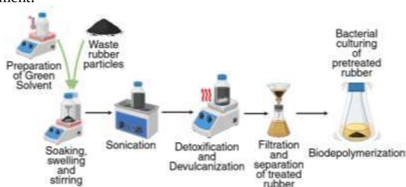
Figure 1. Two-step process for effective rubber degradation
