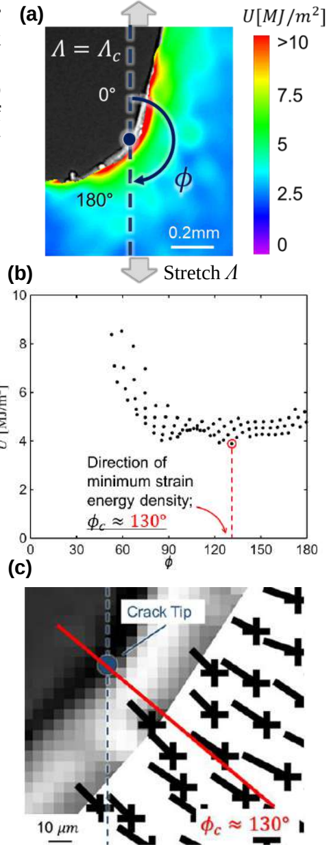
Figure 3(a). Distribution of strain energy density ( U ) around the crack tip at the crack-growth onset ( \lambda = \lambda_c ). (b). Polar plot of U . The center is the crack tip, and the radius is 200\ \mu\text{m} . (c). Distribution of local minor principal strain axis direction at \lambda = \lambda_c . The red line shows the direction of the minimum value of U .
