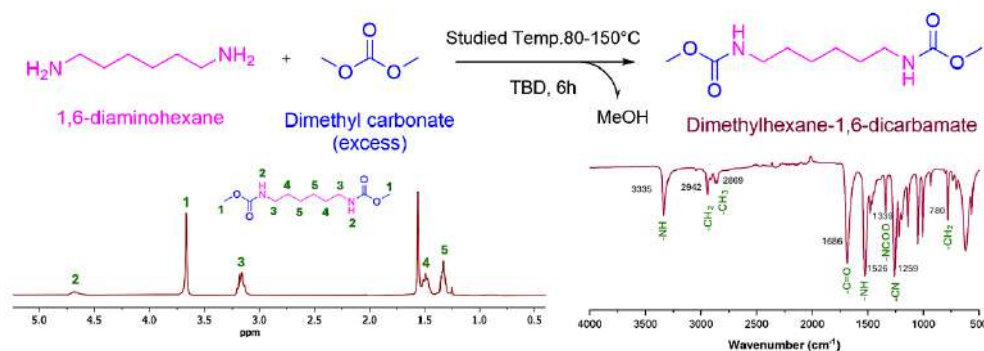
Figure 2. Synthesis and characterization of Dimethylhexane-1,6-dicarbamate
