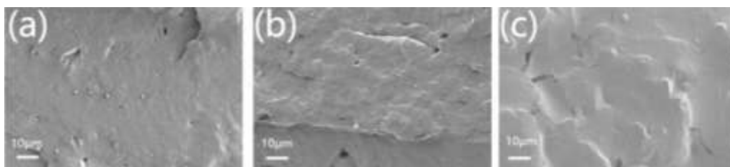
Figure 2. SEM images of (a) NBR-L20, (b) IX-NBR-L20, and (c) HX-NBR-L20.
