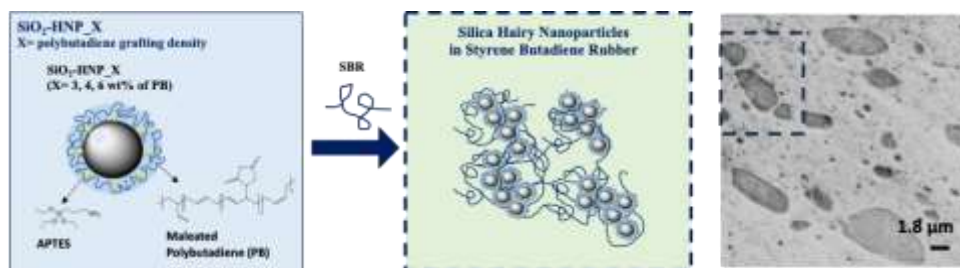
Figure 1. Schematic representation of the HNPs synthesis and their self-assembly in SBR NCs
