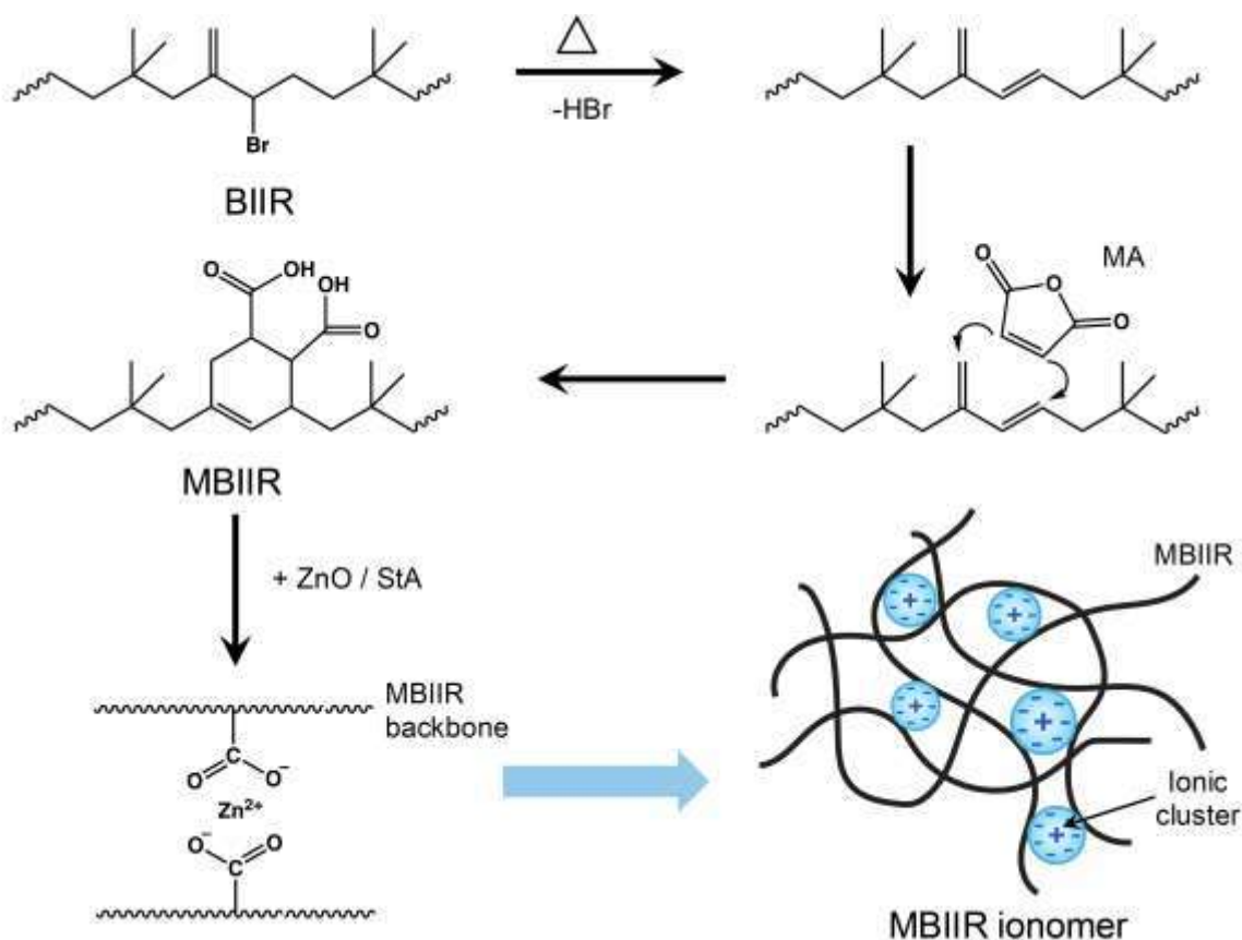
Figure 1. Chemical modification of BIIR with MA and synthesis of MBIIR ionomer
