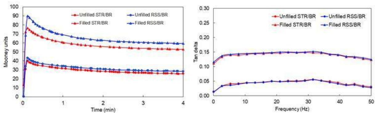
Figure 2. Mooney viscosities and tan delta at 60 °C of unfilled- and HAF-filled NR/BR blends
