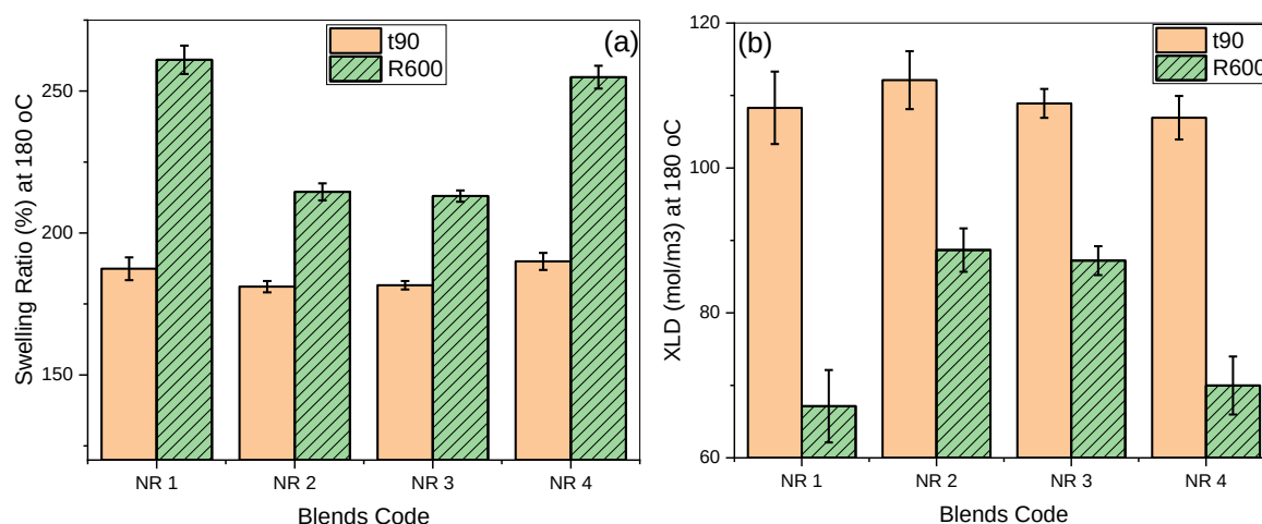
Figure 2. Swelling rates and XLD value of NR series blends at 180 °C with t_{90} and R_{600} times.
