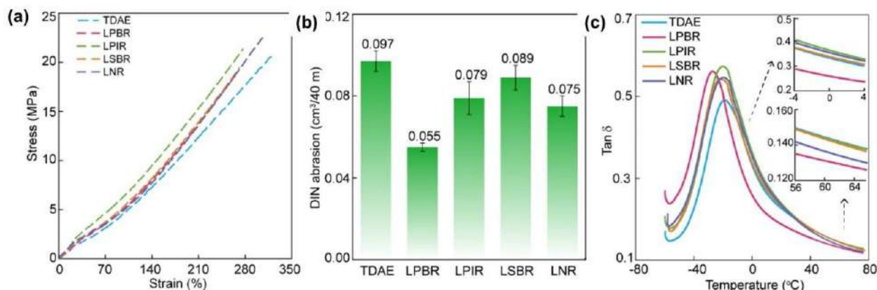
Figure 2. (a) Stress-strain curves of compounds containing TDAE oil and degraded LPRs. (b) DIN abrasion (volume loss) of compounds containing TDAE oil and degraded LPRs. (c) Tan \delta -temperature curves of composites at 0.5% tensile strain.
