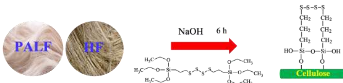
Figure 1. Natural fiber treatment process: PALF or HF was treated by NaOH and then silane 69 for 6 h to link the silane 69 on the surface of natural fibers
