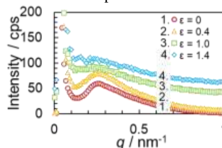
Figure 1. SAXS profiles of SPU during equi-biaxial deformation.
