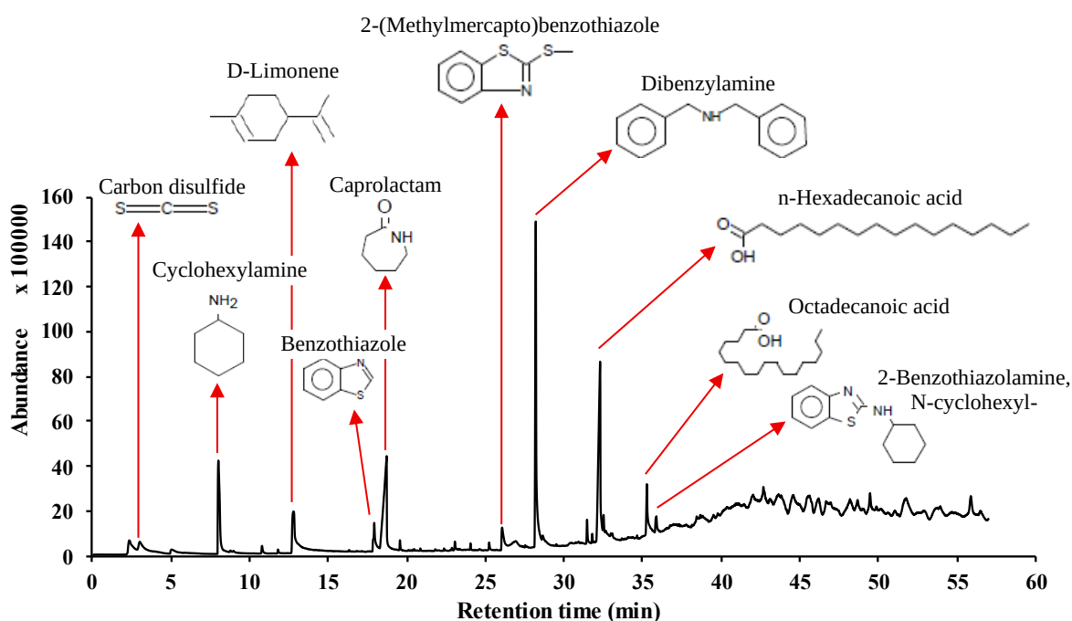
Figure 1. GC-MS chromatogram at 300°C of cured standard Thai rubber 20 (C-STR20)
