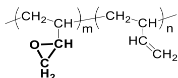
Figure 1. 1,2-Epoxydized Polybutadiene
