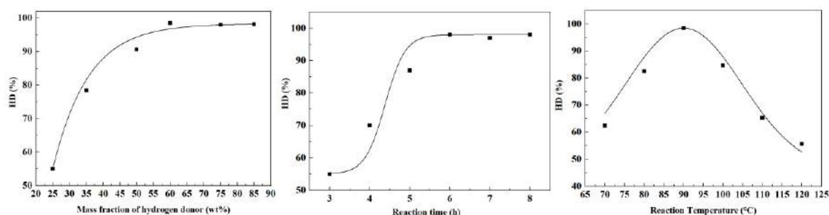
Figure 2. The influence of hydrogen donor concentration, reaction time, and reaction temperature on the hydrogenation of NBR latex
