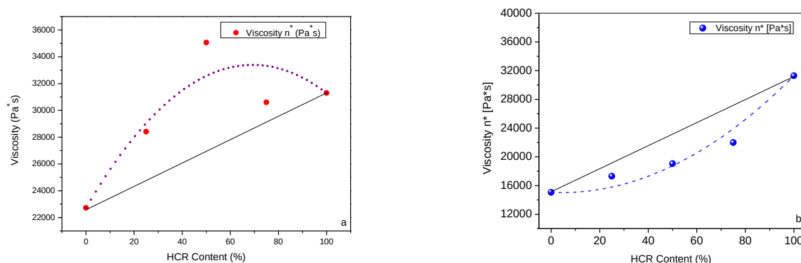
Figure 1. Variation of viscosity of a) ECO/HCR and b) CO/HCR blends with HCR content
