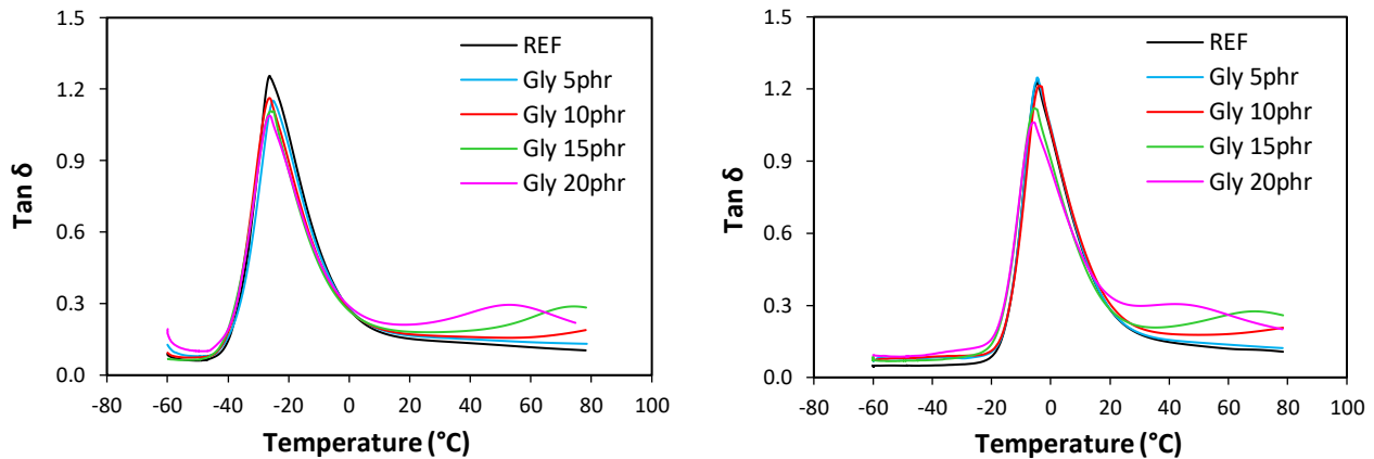
Figure 1. Temperature dependences of loss factor \tan \delta for composites based on SBR (left) and NBR (right)
