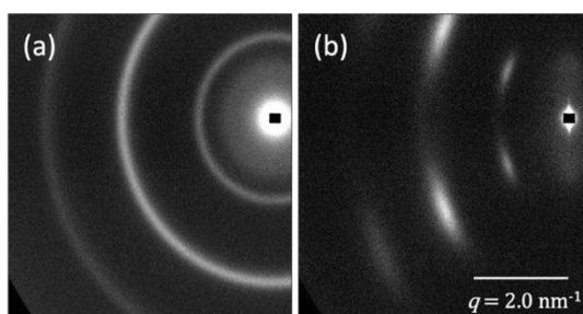
Figure 2. Two-dimensional SAXS patterns of the pressed specimen (a) before stretching and (b) at 10.0-fold uniaxially stretched state.
