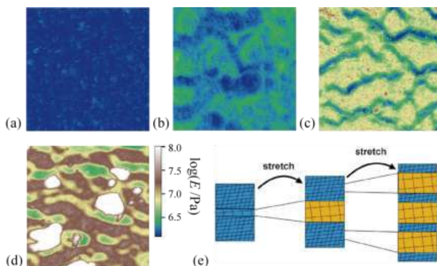
Figure 1. Elastic modulus mappings of IR vulcanizates (a) unstretched; (b) stretched to \lambda = 100\% ; (c) stretched to \lambda = 300\% (d) stretched to \lambda = 500\% . The scan sizes are 1.0 \mu\text{m} \times 1.0 \mu\text{m} . (e) Schematic diagram of the microscopic deformation behavior based on this transformation process.
