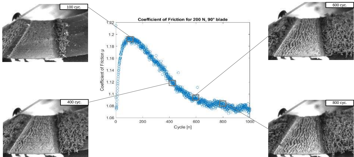
Figure 1. The coefficient of friction evolved over 1000 cycles with a blade with a 90° angle and a 200N normal load.
