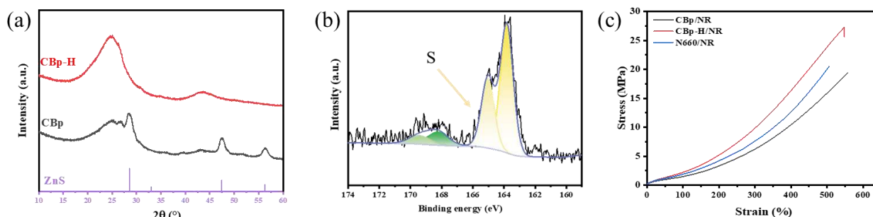
Figure 1. (a) The XRD patterns of CBp and CBp-H; (b) the high-resolution S 2p XPS spectrum of CBp-H; (c) representative stress–strain curves of natural rubber composites reinforced with CBp, N660 and CBp-H.
