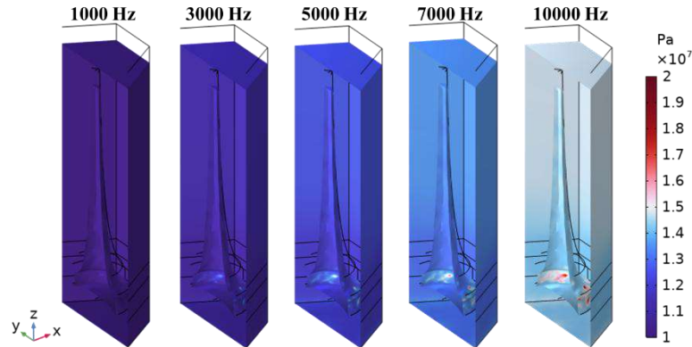
Figure 2. Storage modulus of acoustic coating at different frequencies under 1 MPa pressure
