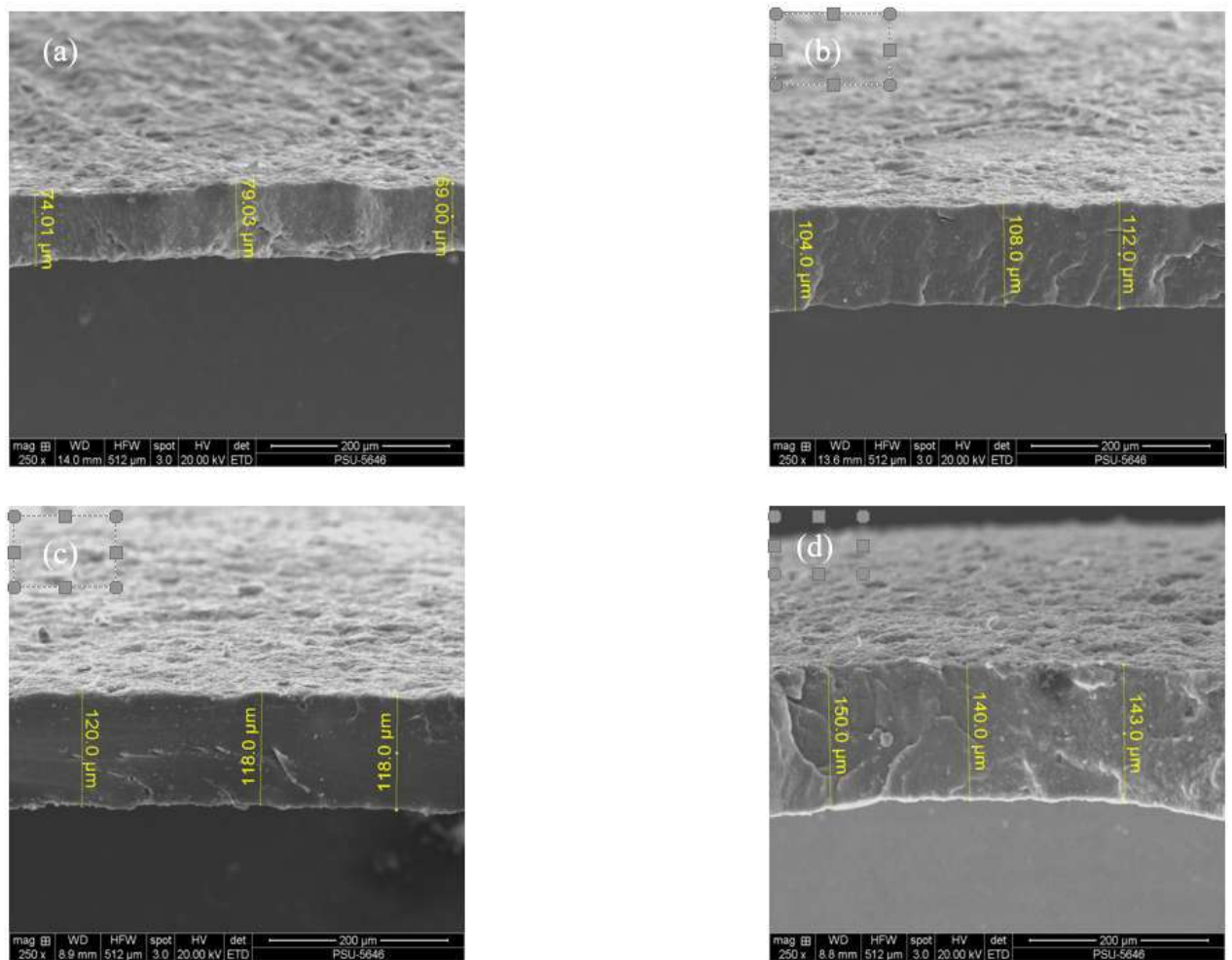
Figure 1. SEM images of vulcanized latex film cross-section by varying the calcium nitrated (N) concentration with solid content (SC) of compound latex (a) N2-SC25, (b) N4-SC25, (c) N8SC35, and (d) N16SC25.
