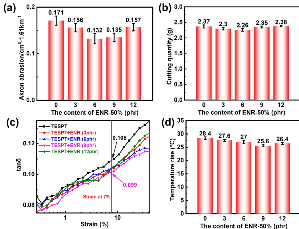
Figure 2. (a) Akron abrasion, (b) cut resistance, (c) curves of tan \delta -strain at 60°C and (d) temperature rise of EUG/NR/SBR nanocomposites with different ENR dosages.
