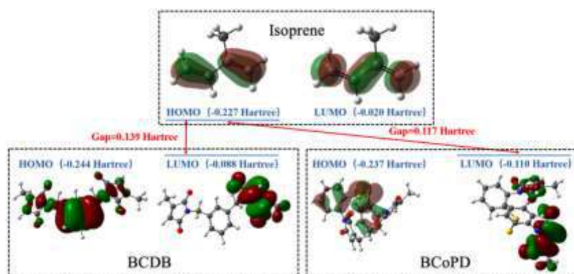
Figure 3. Frontier orbital energy levels of NR (isoprene), BCDB and BCoPD
