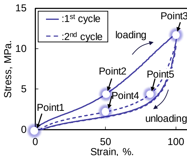
Figure 1. Stress-strain curves.
