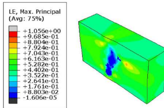
Figure 1. FEM analysis of a Representative Volume Element (RVE) with Periodic Boundary Conditions (PBCs) embedding a reconstructed carbon black (CB) aggregate.
