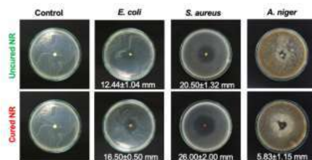
Figure 1. The qualitative antimicrobial activities against E. coli , S. aureus and A. niger of uncured and cured NR films filled with 15 %wt cinnamon oil and controlled samples.
