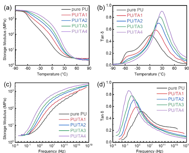
Figure 2. (a) Storage modulus-Temperature curves of bio-PU/TA composites. (b) \tan\delta -Temperature curves of bio-PU/TA composites. (c) Storage modulus- f curves of bio-PU/TA composites. (d) \tan\delta - f of bio-PU/TA composites.
