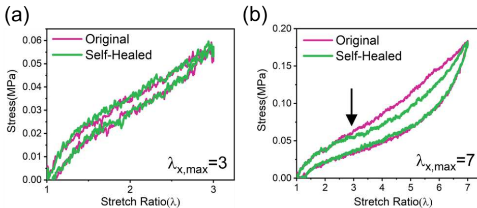
Figure 2. Tensile loading-unloading cycles of the original PAAm-fCNT-2 ( X=3 ) and that after self-healing at (a) \lambda_{x,max}=3 and (b) \lambda_{x,max}=7 .
