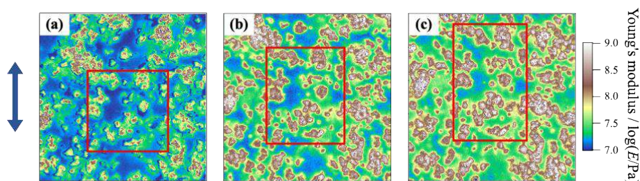
Figure 1. In situ AFM elastic modulus mappings for silica/SBR with TESPT in 1.0 \times 1.0 \mu\text{m} areas under elongation of (a) 0%, (b) 16%, and (c) 45%. Areas in the red frames refer to identical locations.
