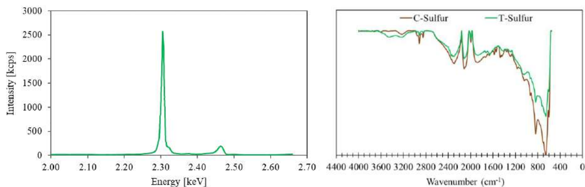
Figure 1. XRF spectrum of treated sulfur sludge (a) and FTIR spectra with various sulfur (b).
