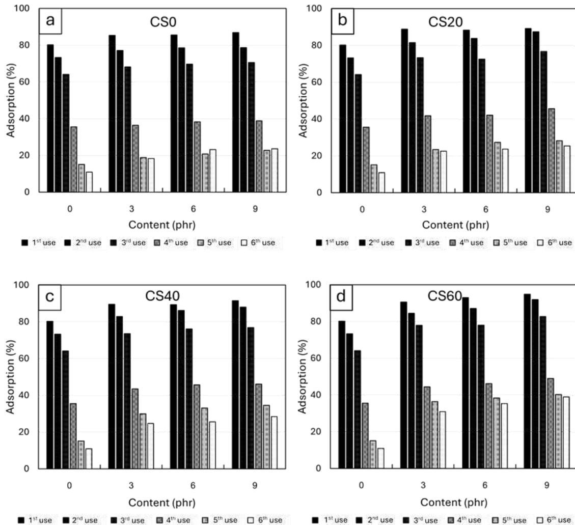
Figure 1. Copper (Cu) adsorption abilities for NRF containing varying contents of (a) CS0, (b) CS20, (c) CS40, and (d) CS60, determined for a total of six cycles of use.
