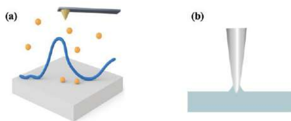
Figure 1. (a) Schematic of SMFS, showing the AFM probe approaching a polymer single chain adsorbed on inorganic surface. (b) Schematic of nano-palpation, depicting the adhesion response during probe retraction from the cross-linked rubber surface.
