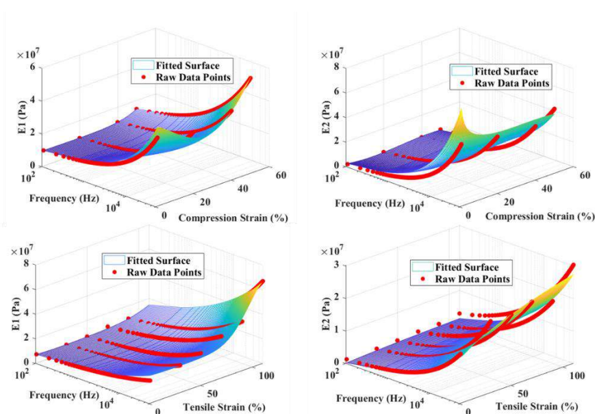
Figure 1. Storage modulus and loss modulus of SBR under different pre-strain
