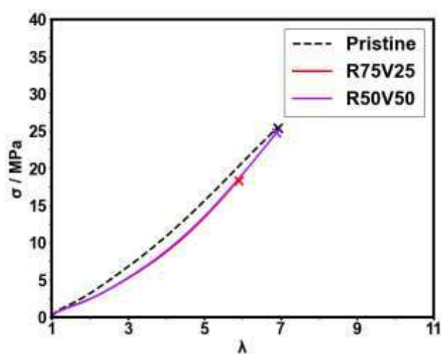
Figure 2. Stress-Extension Ratio curve for the pristine and recycled model filled SEV compounds.
