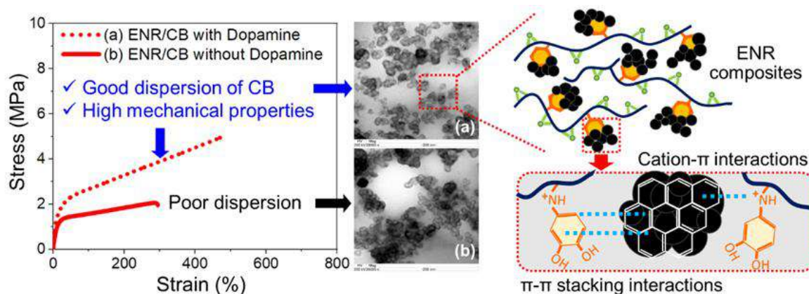
Figure 2. Stress-strain curves, TEM images, and model of the ENR composites with/without D [4].
