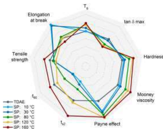
Figure 1. Overall performance of the studied rubber compounds
