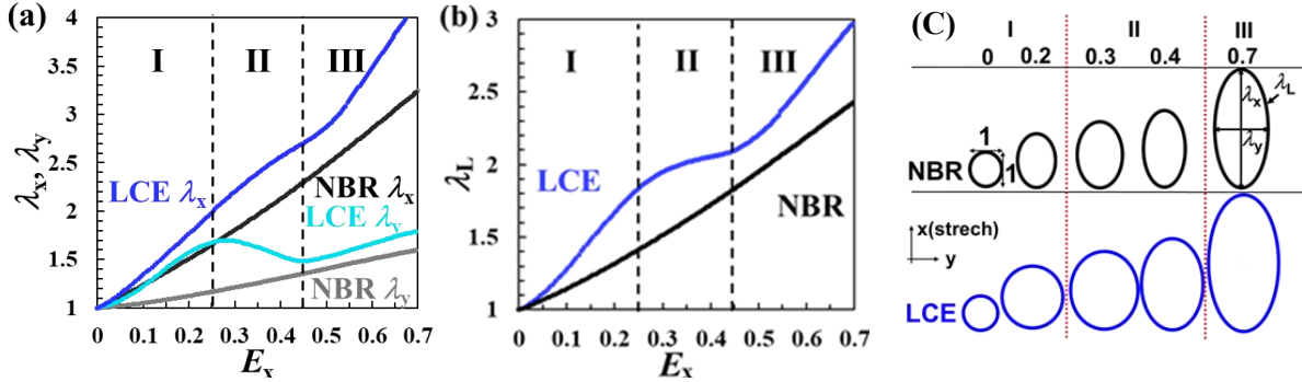
Figure 3 (a) \lambda_x or \lambda_y , (b) \lambda_L as a function of E_x for LCE and NBR and (c) change of the vacancy
