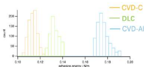
Figure 2. Adhesion energy distribution measured with three types of probes.
