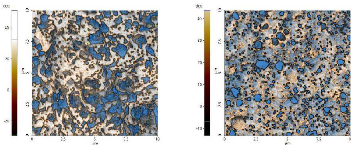
Figure 1. AFM phase images of NR-SR blends with and without (left) compatibilizer. The areas with blue and whitish colors represent NR and SR respectively.
