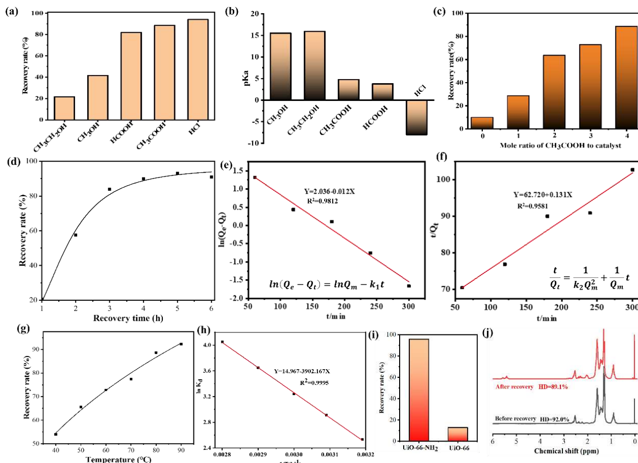
Figure 1. (a) Relationship between additives and recovery rate; (b) pKa values of different additives; (c) Graph showing the relationship between additive dosage and recovery rate; (d) Relationship between recovery rate and time; (e) First-order (f) Second-order kinetic model; (g) Relationship between recovery rate and temperature; (h) Adsorption thermodynamic model; (i) Recovery rates of different types of adsorbents; (j) HNBR nuclear magnetic spectra before and after catalyst recovery
