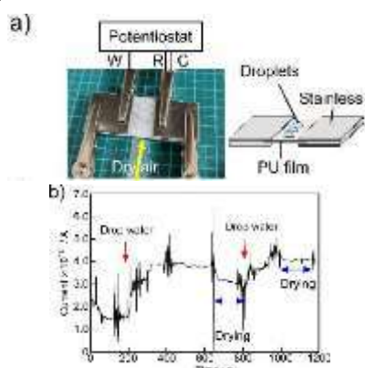
Figure 4. a) Photo and cartoon of a measurement cell for the moisture-dependent electrical conductivity measurement. b) Time course of electric current value: bias voltage, 2.0 V.
