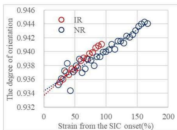
Figure 2. The degree of orientation as a function of strain from the SIC onset
