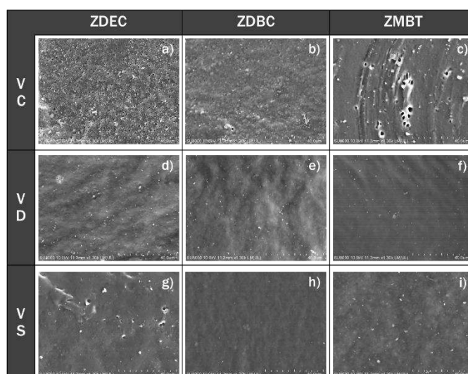
Figure 2. SEM images of a cross-section of finger cots prepared from various latex types and accelerators.
