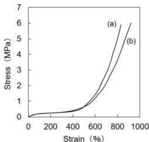
Figure 2 Stress-strain curve of (a) NR-50-control and (b) NR(150-45-LS).
