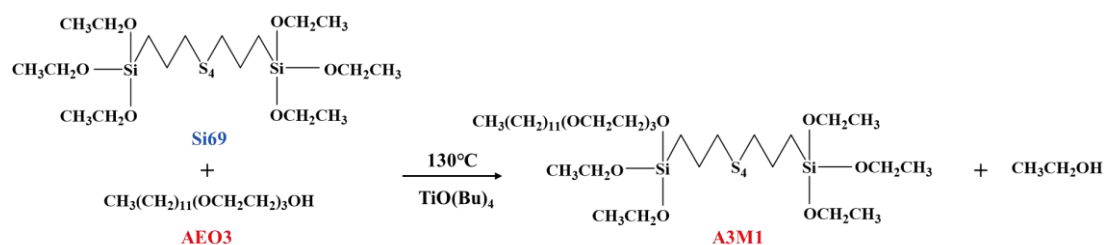
Figure 1. Synthesis reaction of A3M1.
