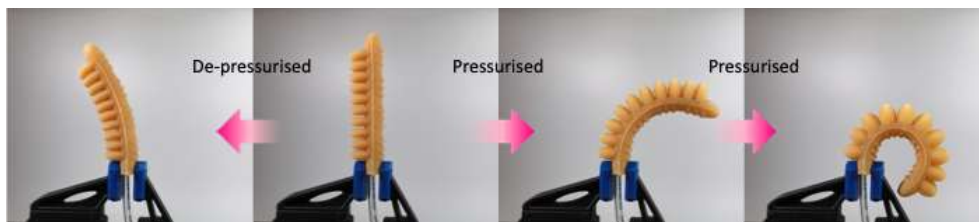
Figure 2. Actuation mechanism of NR soft robotics actuator under negative and positive air pressure
