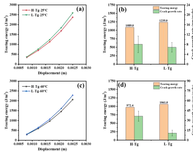
Figure 2. (a) and (c) Tearing energy - displacement curve; (b) and (d) Tearing energy and Crack growth rate at 20% deformation
