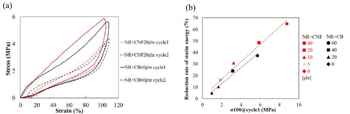
Figure 4. Repeated tensile test (a) strain-stress curve at 100% tensile and (b) 100% modulus in 1 st cycle vs. hysteresis loss
