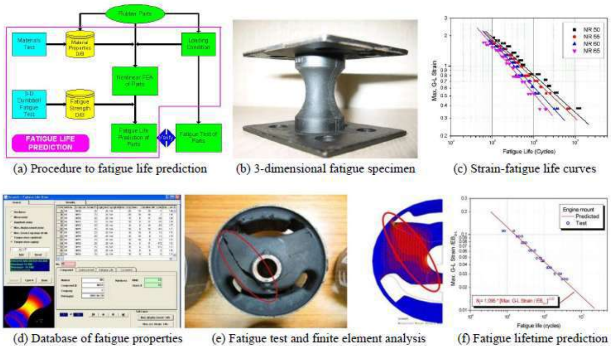
Figure 2. Fatigue lifetime prediction of rubber components
