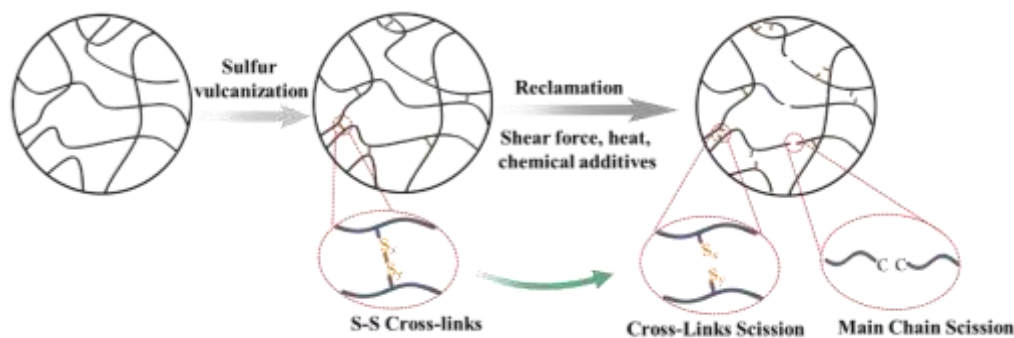
Figure 1. The bond-breaking mechanism within the crosslinked network during the reclaimed process
