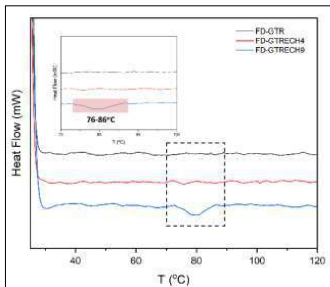
Figure 2. DSC thermograms of FD-GTR and FD-GTRECHs
