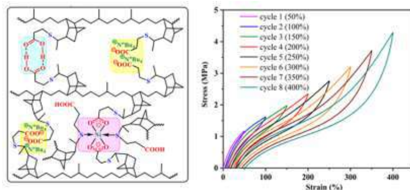
Figure 2. rc EPDM networks with noncovalent cross-linking sites and their cyclic tensile test curves
