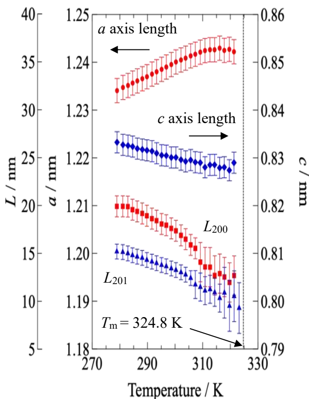
Fig.1 Temperature dependence of lattice constants ( a , c ) and crystallite size ( L_{200} , L_{201} )
