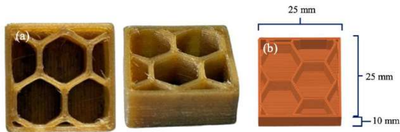
Figure 1. (a) 3D-printed structures fabricated using a TPU/NR-ENR 95/5 blend containing 3 phr of ENR, and (b) 3D model of the honeycomb structure.
