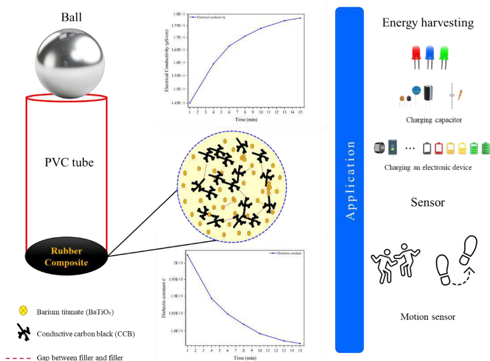
Figure 1. Proposed dropping ball test, mechanism, and application of composites
