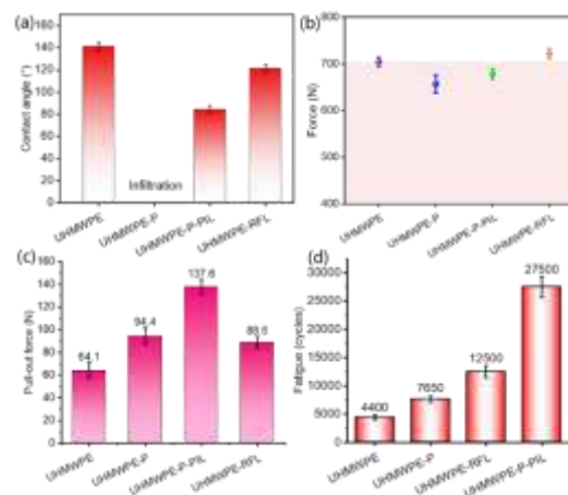
Figure 2. (a) Water contact angle, (b) breaking force, (c) static interfacial adhesion, and (d) dynamic interfacial adhesion of modified fibers.
