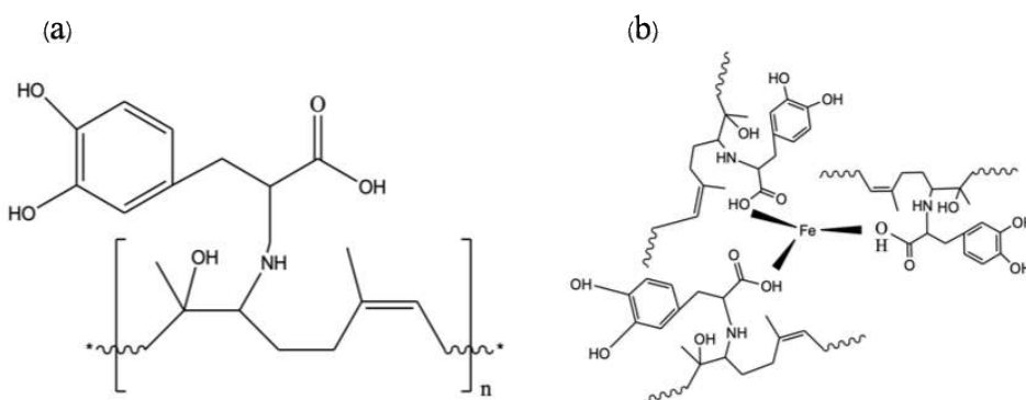
Figure 1. Chemical structure of ENR with DOPA (a), and ENR with DOPA and Fe (b)
