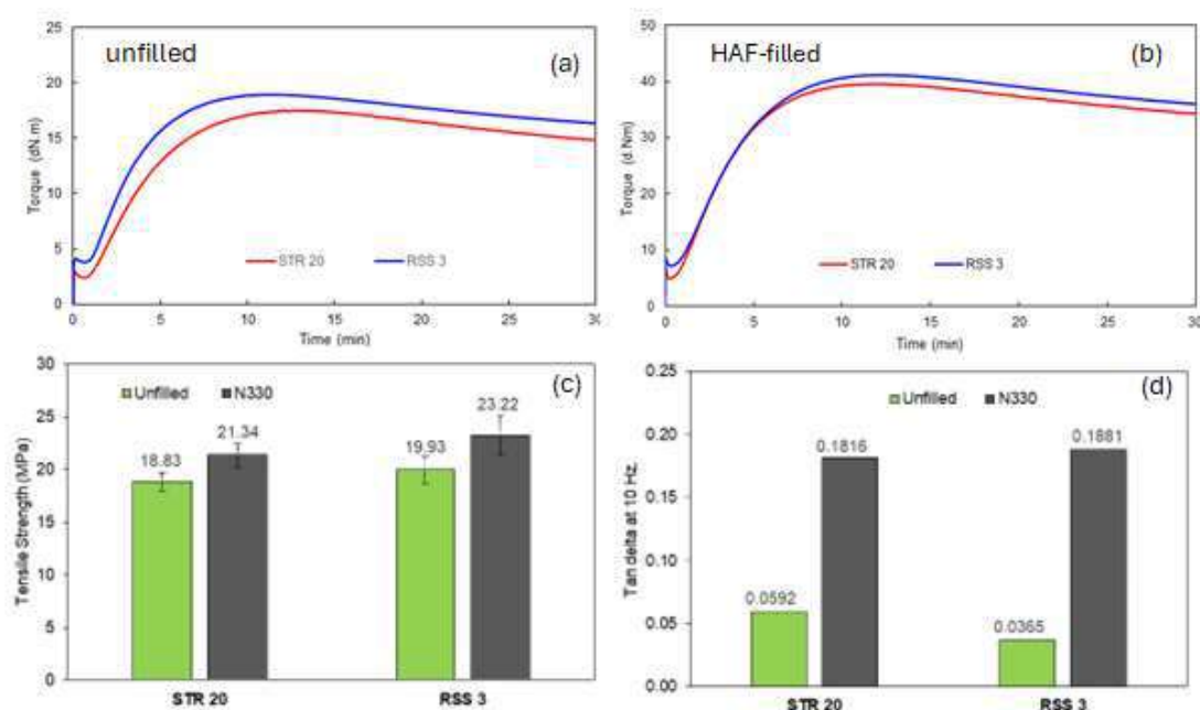
Figure 1. Properties of unfilled- and HAF-filled-compounds comparing the use of STR20 vs. RSS3
