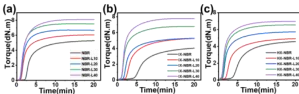
Figure 1. Vulcanization curve diagram of (a) NBR-L, (b) IX-NBR-L, and (c) HX-NBR-L.
