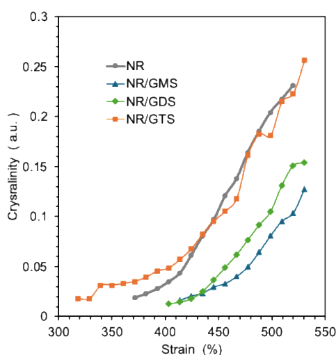
Figure 2. Crystallinity index of NR, NR/GMS, NR/GDS, and NR/GTS as a function of strain.
