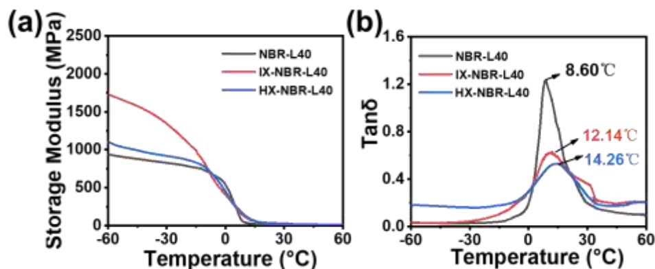
Figure 4. (a) Storage modulus and (b) Tan \delta curves of XNBR/lignin compounds with three different carboxyl contents.
