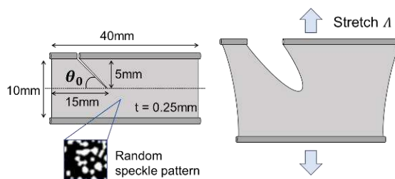
Figure 1. Geometry of crack growth experiment
