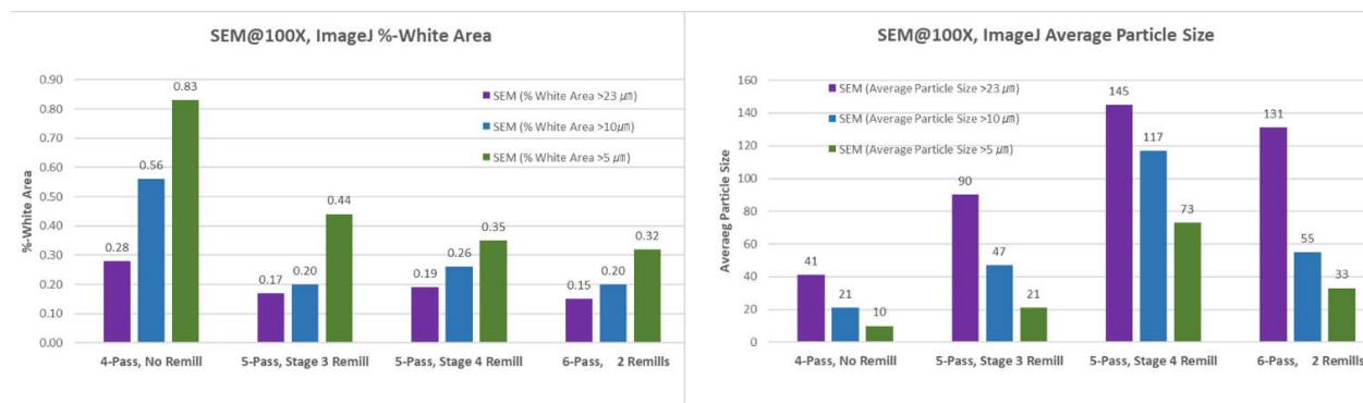
Figure 5. %-White areas (left) and Average particle sizes (right) of four difference mix sequences.
