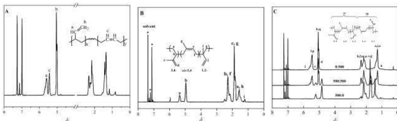
Figure 2. 1 H NMR spectra of polybutadiene (A), polyisoprene (B) and butadiene-isoprene block copolymer (C)
