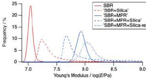
Figure 2. Histogram of Young's modulus for matrix and interface.
