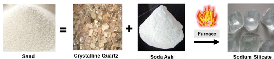
Figure 1. Dry (Furnace) Process to make Sodium Silicate from Minerals (Crystalline Quartz).
