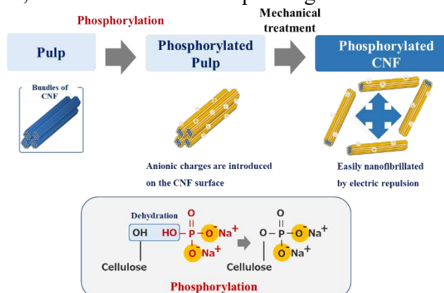
Figure 1. Schematic of the phosphorylated CNF manufacturing process
