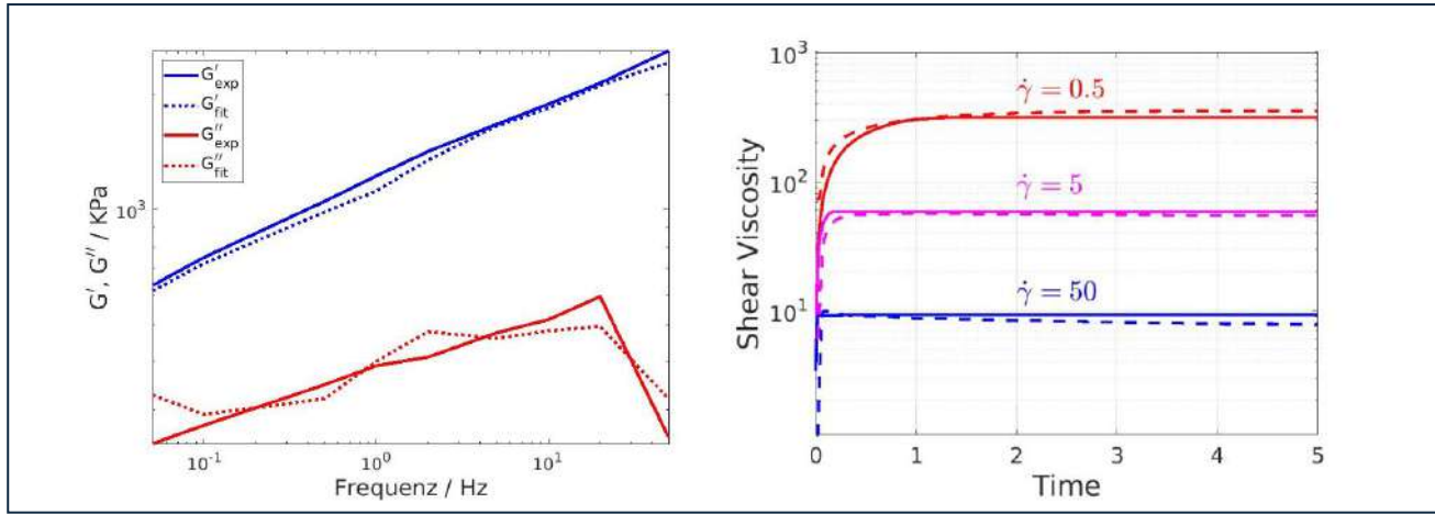
Figure 1: SBR material at T=80^\circ : (Left) G' ( R^2=0.995 ) and G'' ( R^2=0.821 ) fitting with the experimental data. (Right) Shear viscosity with three different values of shear rate ( R^2=0.0689, 0.841, 0.051 ).
