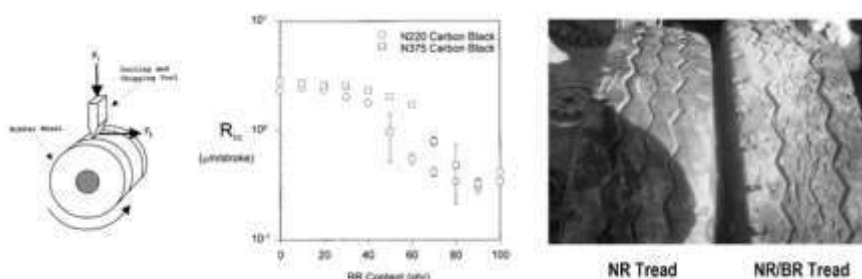
Figure 1. The laboratory cutting and chipping test (left) and truck/bus tire test on a harsh road condition (right) [reprinted from reference 3].
