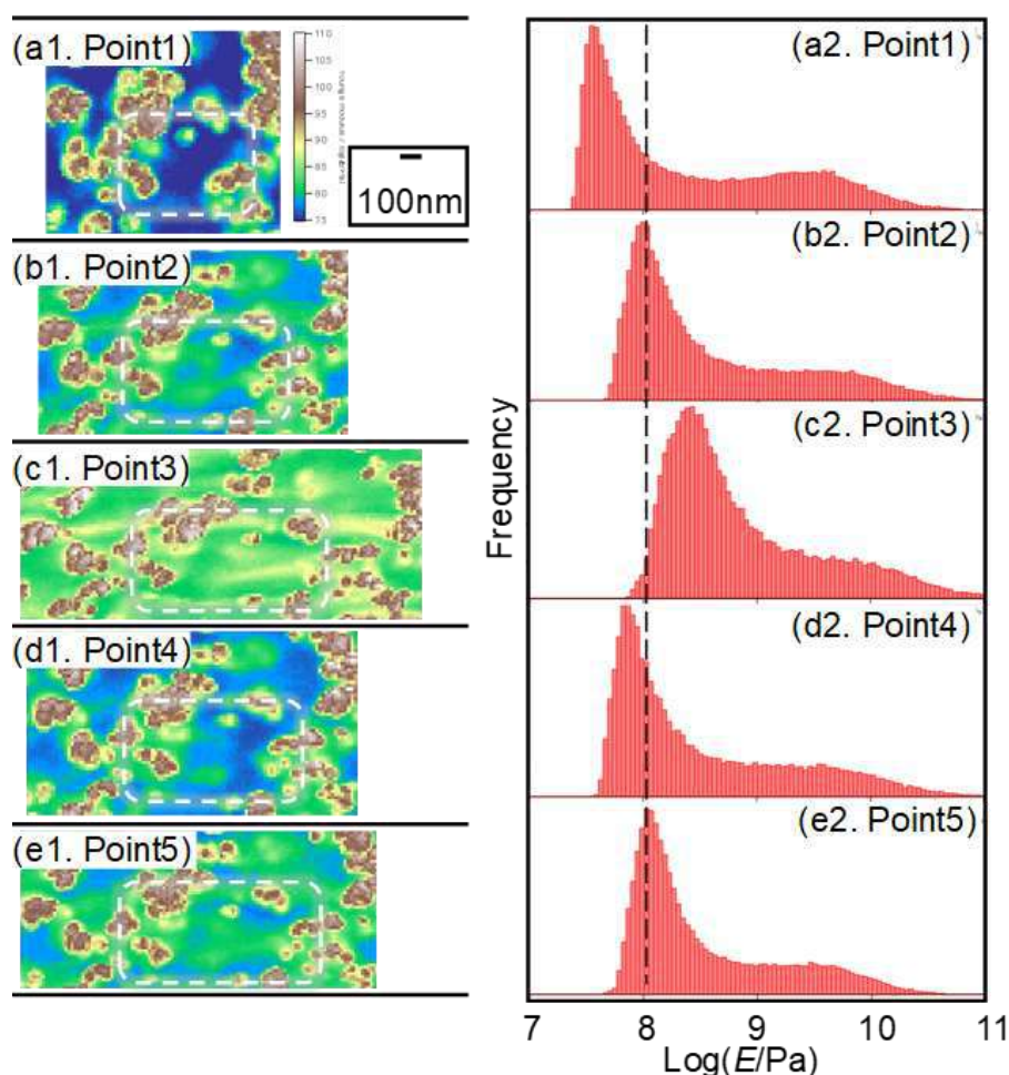
Figure 2. Young's modulus mapping and the corresponding histograms for 26.6 vol% CB/EPDM of (a1, a2) Point1, (b1, b2) Point2, (c1, c2) Point3, and (d1, d2) Point4. The stretching direction was crosswise in the Young's modulus mapping.
