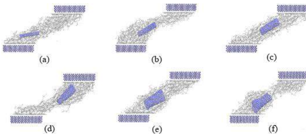
Figure 2. Shear models of CNTs/EUG composites with different CNTs diameters. (a) D2.71-CNTs; (b) D5.42-CNTs; (c) D8.14-CNTs; (d) D10.85-CNTs; (e) D13.56-CNTs; (f) D16.27-CNTs
