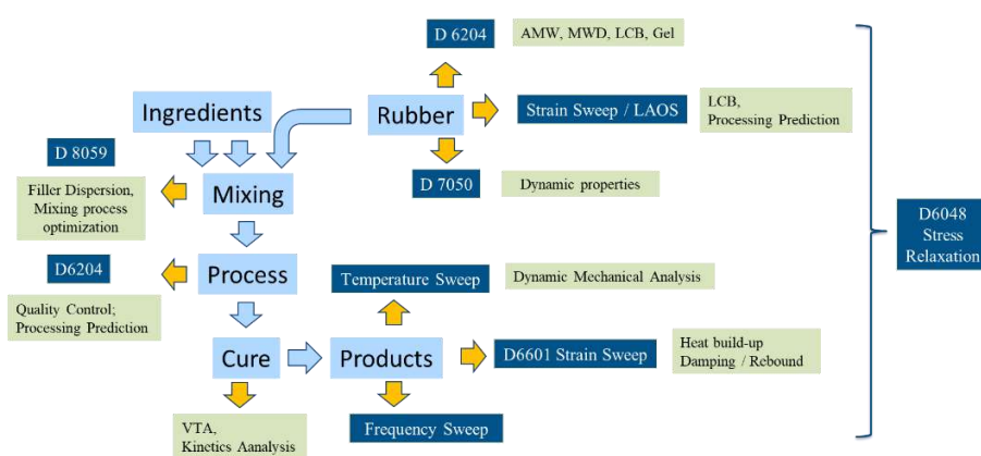
Figure 2. Establishing control on every step of the rubber manufacturing process
