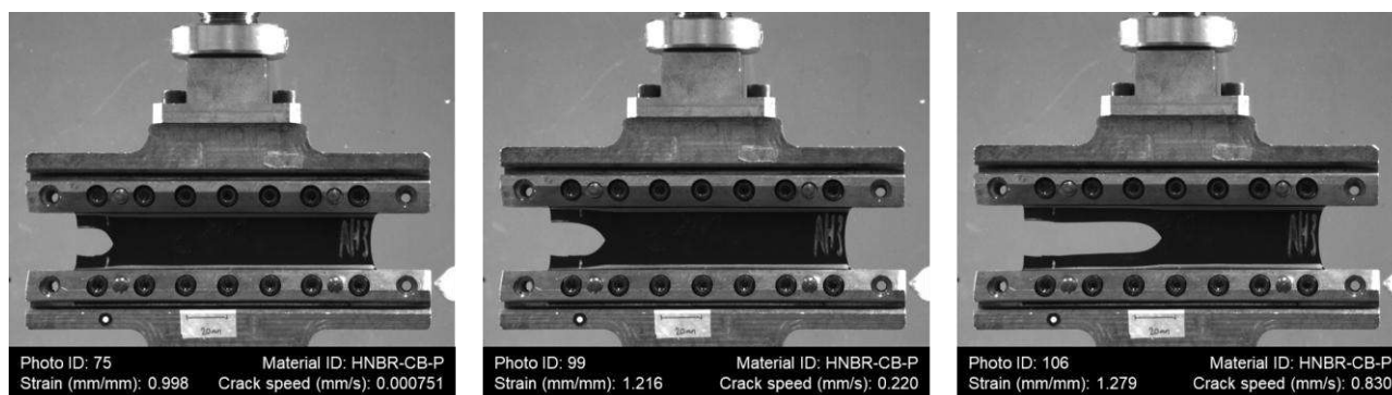
Figure 1: Examples of photographs taken during pure shear testing at various instances. The instantaneous strain and calculated crack speed are shown in each image.
