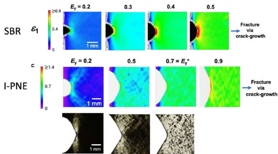
Figure 2. Evolutions of spatial distribution of principal maximum true strain ( \epsilon_1 ) during quasi-static tensile tearing tests for SBR and I-PNE at various applied macroscopic true strains ( E_y ). Corresponding optical transmission images are displayed alongside the strain maps. The turbid and transparent regions represent the polydomain and monodomain textures, respectively.[7]
