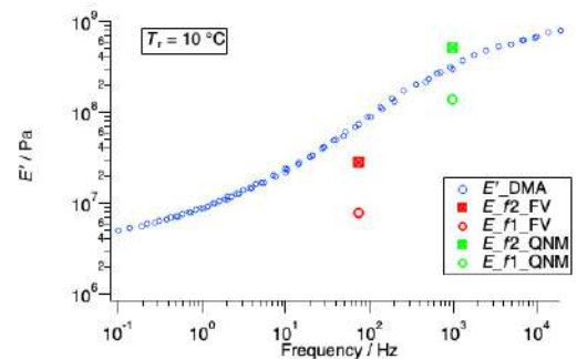
Figure 3. Comparison of macroscopic storage modulus and AFM modulus for SBR+MPR+Silica systems (single kneading).
