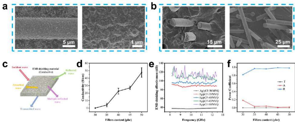
Figure 2. (a) SEM images of Ag/pCF; (b) SEM images of Ag/pCF/MVQ composites; (c) The EMI shielding mechanism of Ag/pCF/MVQ composites; (d) The conductivity of Ag/pCF/MVQ composites; (e) The EMI shielding effectiveness of Ag/pCF/MVQ composites; (f) The power coefficients of of Ag/pCF/MVQ composites
