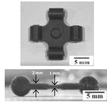
Figure 1. Cross-shaped specimen for the biaxial elongation.
