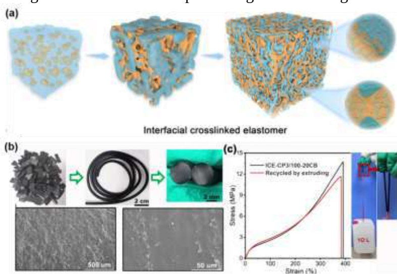
Figure 1. (a) Scheme for the formation process of the skeletal network via granule percolation and interfacial crosslinks. (b) Extrudable reprocessing of multiphase rubbers and their microscopic morphology on the surface/cross-section. (c) Tensile properties of the extruded sample and its load-bearing demonstration.
