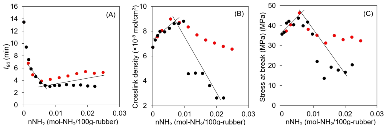
Figure 1. Plot of (A) optimal vulcanization time ( t_{90} ), (B) Crosslink density, and (C) Stress at break versus mole of NH 2 group in 100 g-rubber (Black: DP-ODA; Red: DP-OMDA)
