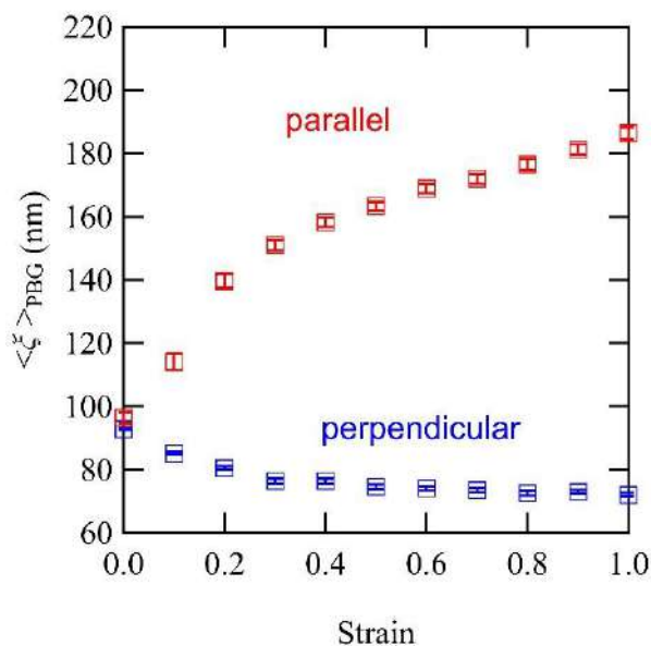
Figure 3 The correlation distance of aggregate in the parallel and perpendicular direction to the elongation as a function of strain
