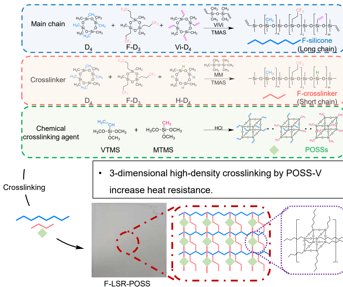
Figure 1. Schematic of all processes for synthesizing fluorosilicone and manufacturing liquid silicone rubber.
