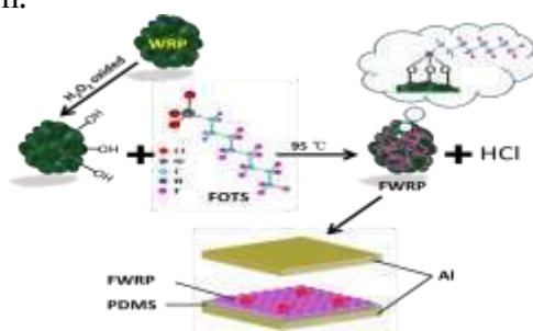
Figure 1. Schematic diagram of surface fluorinated modification for the wasted rubber powder (WRP) by using trichloro (1H,1H,2H,2H-perfluorooctyl) silane (FOTS) as negative electrodes of triboelectric nanogenerators
