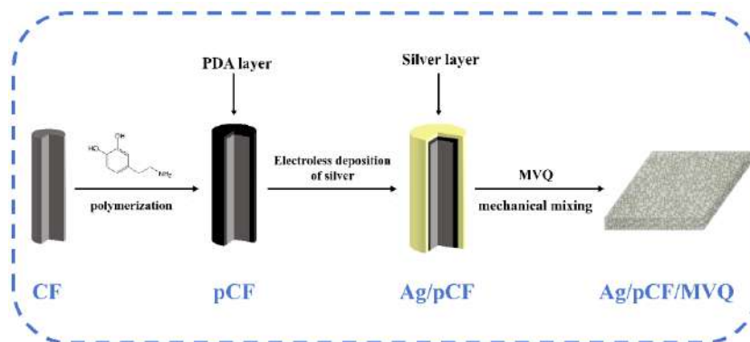
Figure 1. Process for the preparation of Ag/pCF/MVQ composites
