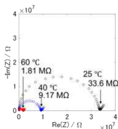
Figure 3. Nyquist diagrams of AC impedance of DES-containing PU. The resistance values in the figure are originated from ionic conduction.
