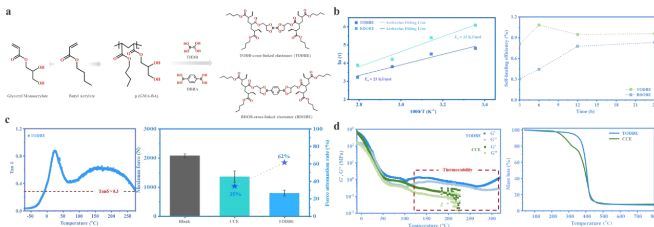
Figure 3. Synthesis and functional performance of the TODBE. (a) Synthesis procedure of TODBE. (b) Activation energy and self-healing efficiency of TODBE relative to BDOBE. (c) Loss factor and anti-impact properties of TODBE. (d) Thermostability of TODBE compared with the covalently cross-linked sample.
