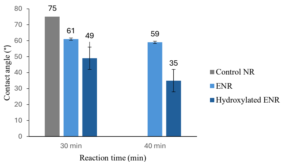
Figure 1. Contact angle measurements of ENR and Hydroxylated ENR obtained at reaction times of 30 and 40 minute.
