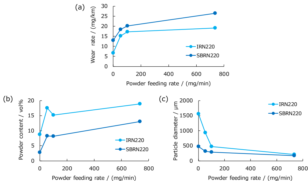
Figure 2. The effect of powder feeding rate on wear rate (a), powder content (b), and particle diameter (c).
