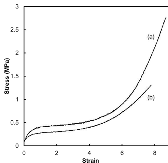
Figure 1. Stress-strain curves of (a) HANR, (b) the 3 rd cream after centrifugation
