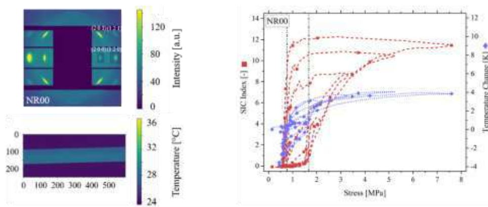
Figure 2. WAXS and IR data representing the SIC behavior of NR under cyclic loading (from [4]).
