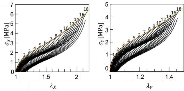
Fig. 3. Nominal stress ( \sigma ) - stretch ( \lambda ) relations in cyclic loading tests of un-equi biaxial elongation (10:4).
