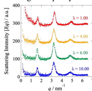
Figure 3. Changes in the one-dimensional SAXS profiles with stretching ratio ( \lambda ) for the pressed specimen.
