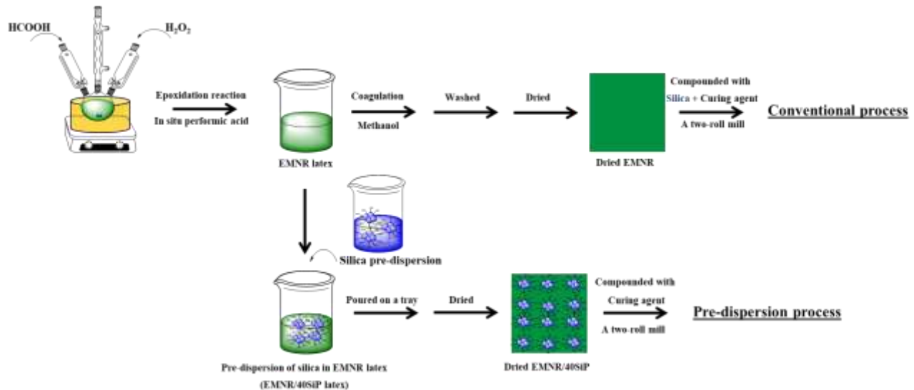
Figure 1. Diagram for preparation of EMNR filled with silica by pre-dispersion process compared with conventional process
