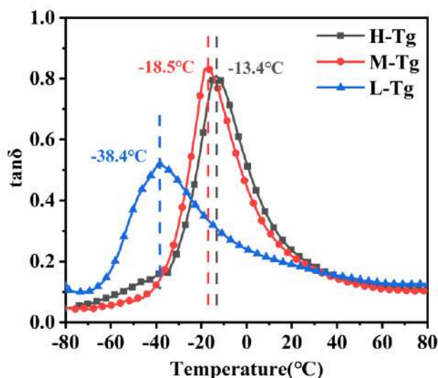
Figure 1. Loss factor versus temperature for different T g rubber composites
