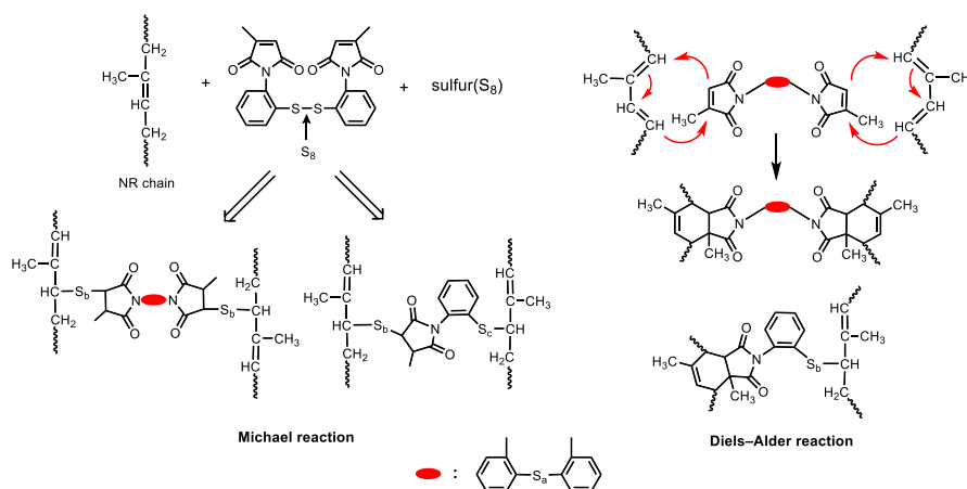
Figure 2. Reaction mechanism of BCoPD with NR
