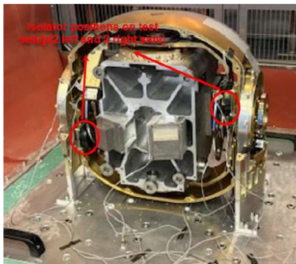
Figure 2. Assembly of the Test Setup on Shaker with Temperature Cabinet
