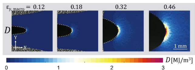
Fig. 5. Development of calculated spatial distributions of D around a crack-tip during crack opening.
