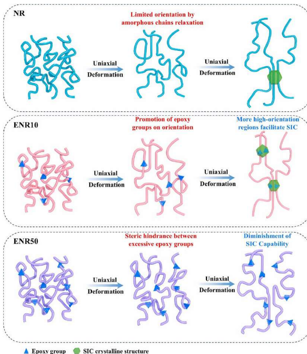
Figure 1. Proposed pathway of microstructure evolution during stretching of NR, ENR10, ENR50.
