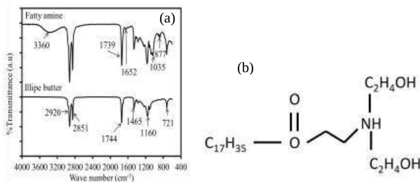
Figure 1. FTIR fatty amine compared to illipe butter (a), possible structure of fatty amine (b)
