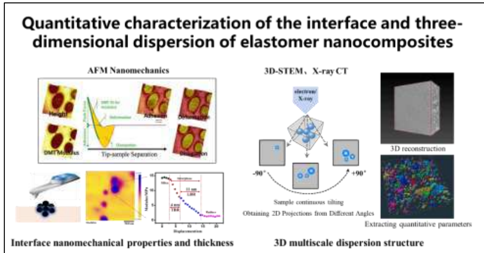
Figure 1. Quantitative characterization of the interface and three-dimensional dispersion of elastomer nanocomposites
