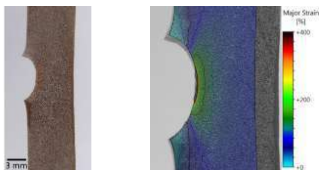
Figure 1. Strain field analysis at the crack tip of a pre-notched NR specimen (from [2]).
