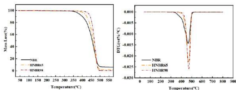
Figure 3. TG and DTG curves of the original rubber and HNBR latex with hydrogenation degrees of 65% and 98%
