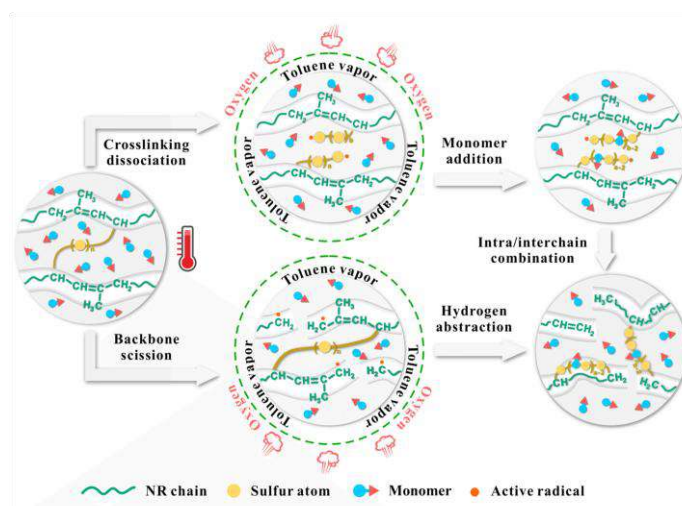
Figure 1. Schematic of the pyrolysis and functionalization of vulcanizates via the dynamic covalent polymerization process.
