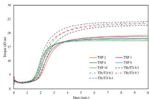
Figure 2. Cure curves of the rubber compounds
