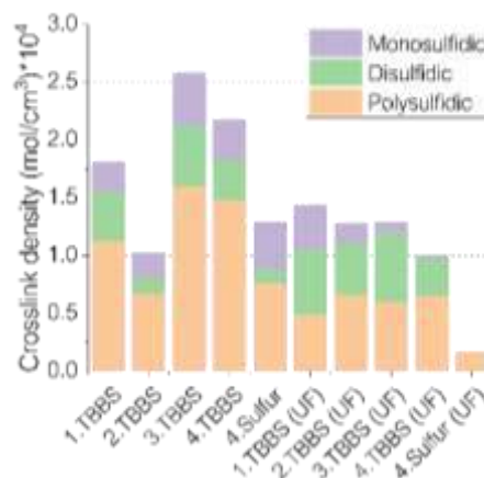
Figure 1. Crosslink structure of both filled and unfilled compounds.
