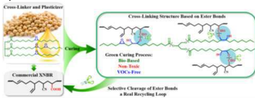
Figure 2. The cross-linking strategy based on ESO for XNBR via epoxy-acid reaction
