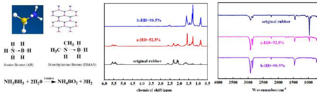
Figure 1. The structure of ammonia borane and dimethylamine borane; ^1\text{H} NMR and IR spectra of NBR latex hydrogenation using (a) AB and (b) DMAB as hydrogen donors
