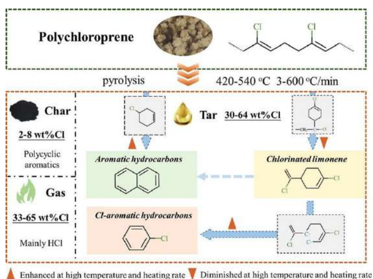
Figure 1. Pyrolysis of untreated polychloroprene (original PCR): Chlorine distribution in solid, liquid, and gas phases
