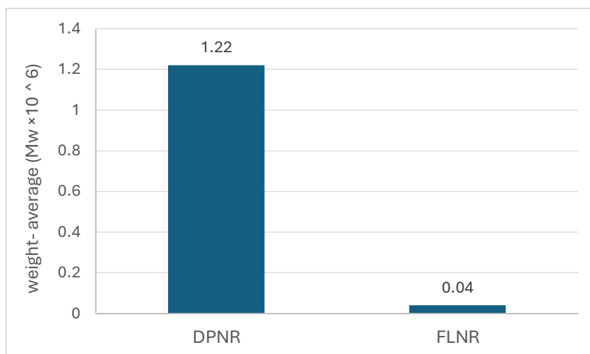
Figure 1. Molecular weight reduction of NR after TiO 2 -HGB-assisted UV-A irradiation.
