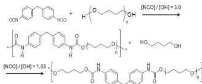
Figure 2. Synthesis scheme for PU by prepolymer method.
