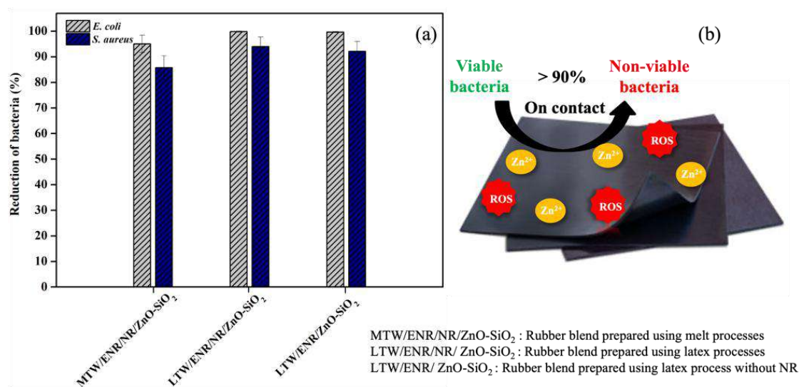
Figure 1. (a) Antibacterial activity of TW/ENR/ZnO-SiO 2 blends with and without NR prepared using melt and latex processes against E.coli and S. aureus ; (b) Proposed mechanism of antibacterial action of the TW/ENR/ZnO-SiO 2 blend with and without NR, illustrating the release of Zn 2+ ions and generation of reactive oxygen species (ROS), leading to bacterial inactivation upon contact.
